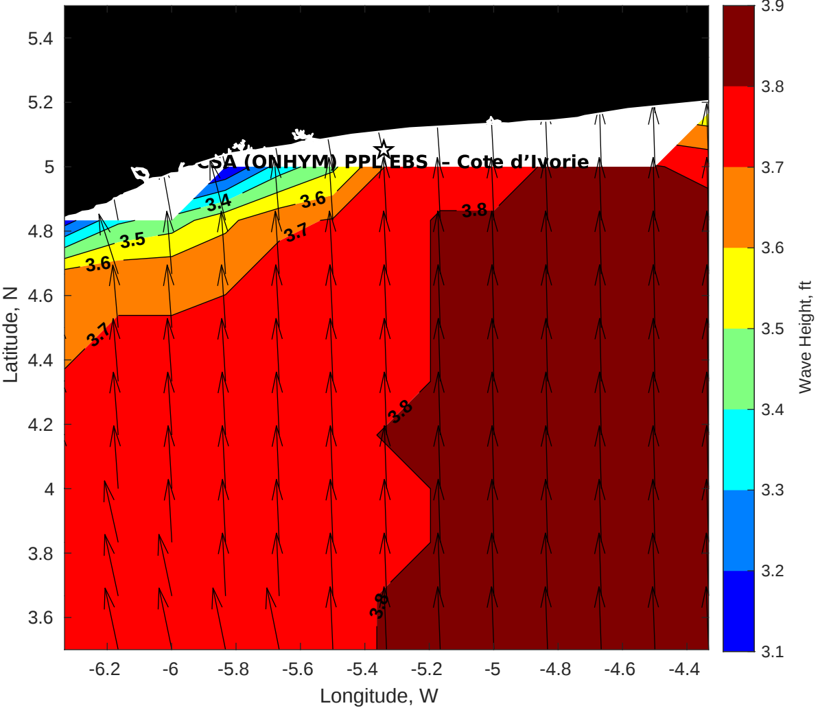
Wave Height (ft) for CSA (ONHYM) PPL EBS - Cote d'Ivoire at 20-Apr-2025 09:00:00
