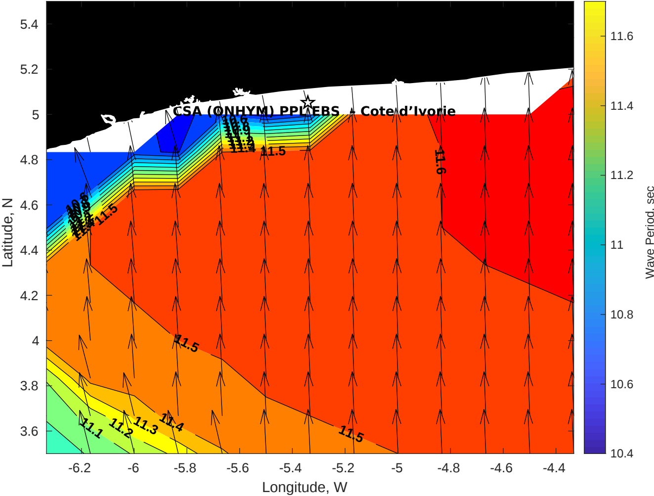
Wave Period (sec) for CSA (ONHYM) PPL EBS - Cote d'Ivoire at 20-Apr-2025 09:00:00
