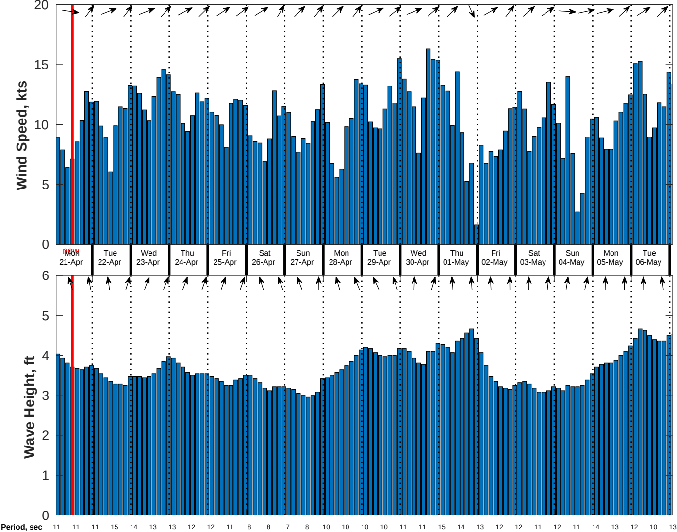
Wind & Wave Forecast for CSA (ONHYM) PPL EBS - Cote d'Ivoire from 20-Apr-2025 01:00:00 to 06-May-2025 01:00:00
