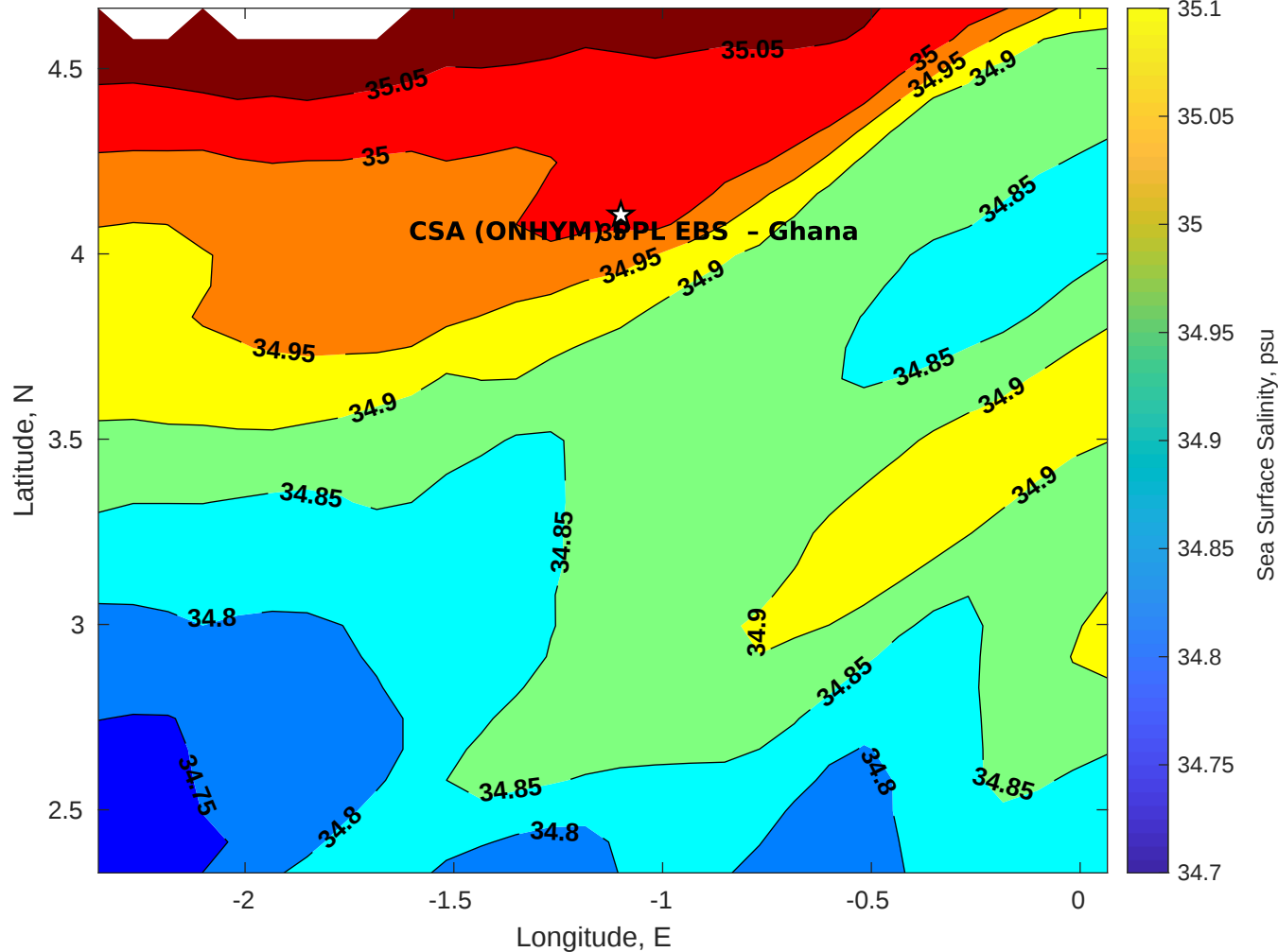
Surface Salinity for CSA (ONHYM) PPL EBS - Ghana at 19-Apr-2025 00:00:00
