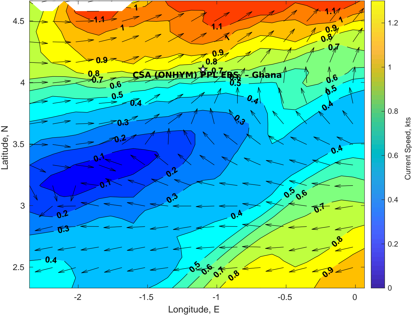
Surface Currents for CSA (ONHYM) PPL EBS - Ghana at 19-Apr-2025 00:00:00
