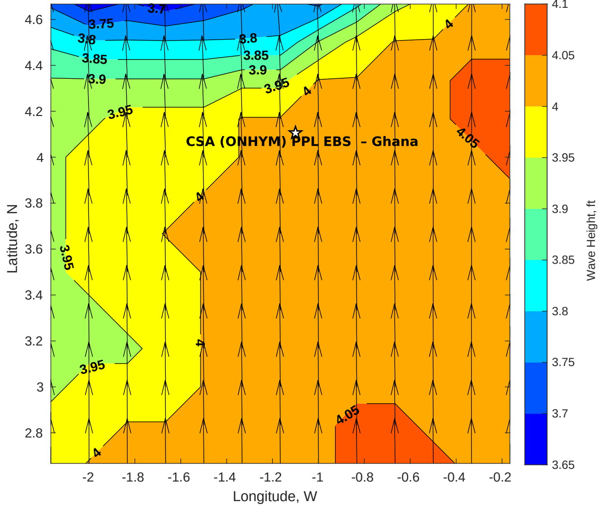
Wave Height (ft) for CSA (ONHYM) PPL EBS - Ghana at 20-Apr-2025 09:00:00
