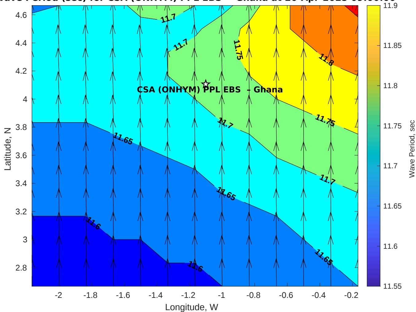
Wave Period (sec) for CSA (ONHYM) PPL EBS - Ghana at 20-Apr-2025 09:00:00
