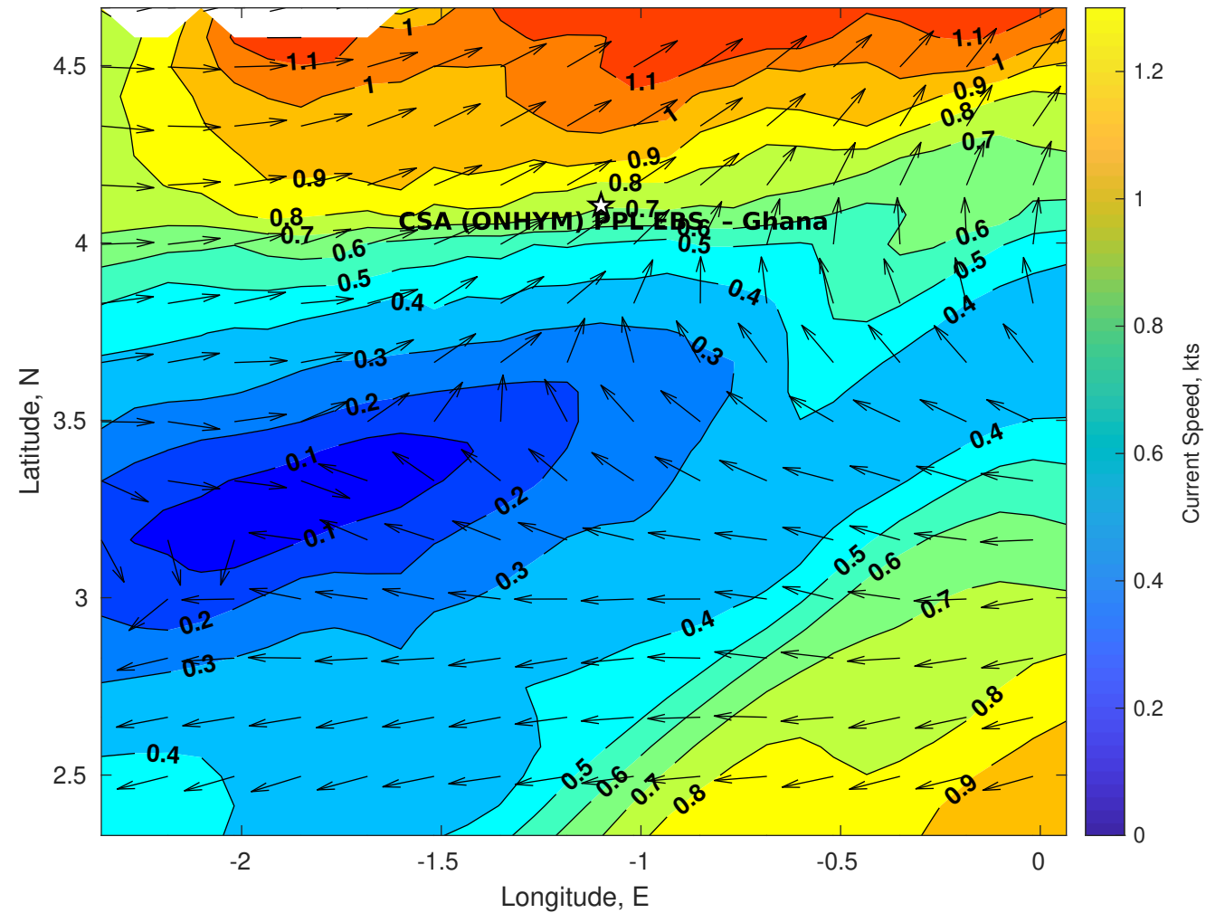
Surface Currents for CSA (ONHYM) PPL EBS - Ghana at 19-Apr-2025 00:00:00
