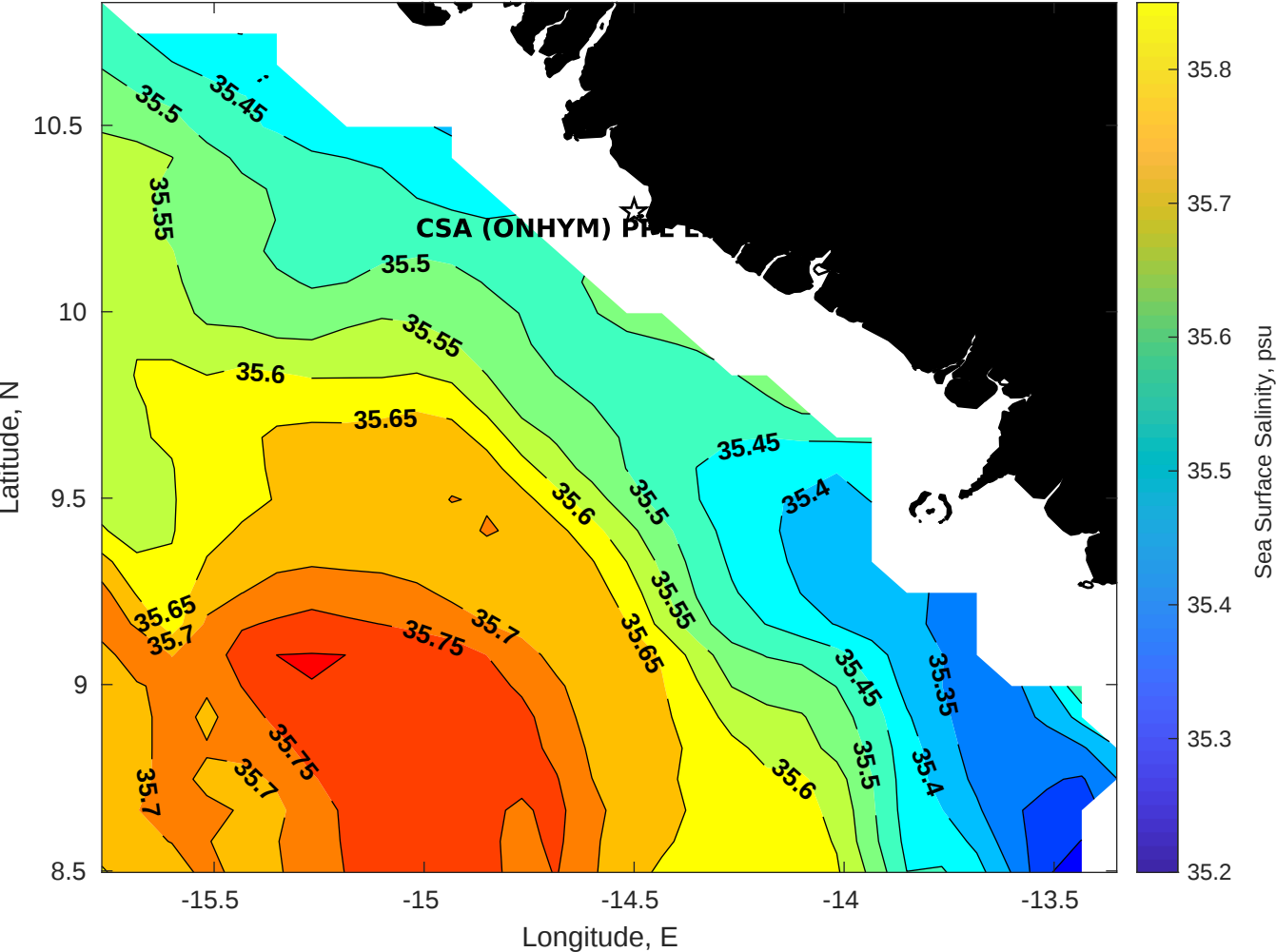
Surface Salinity for CSA (ONHYM) PPL EBS - Guinea at 19-Apr-2025 00:00:00
