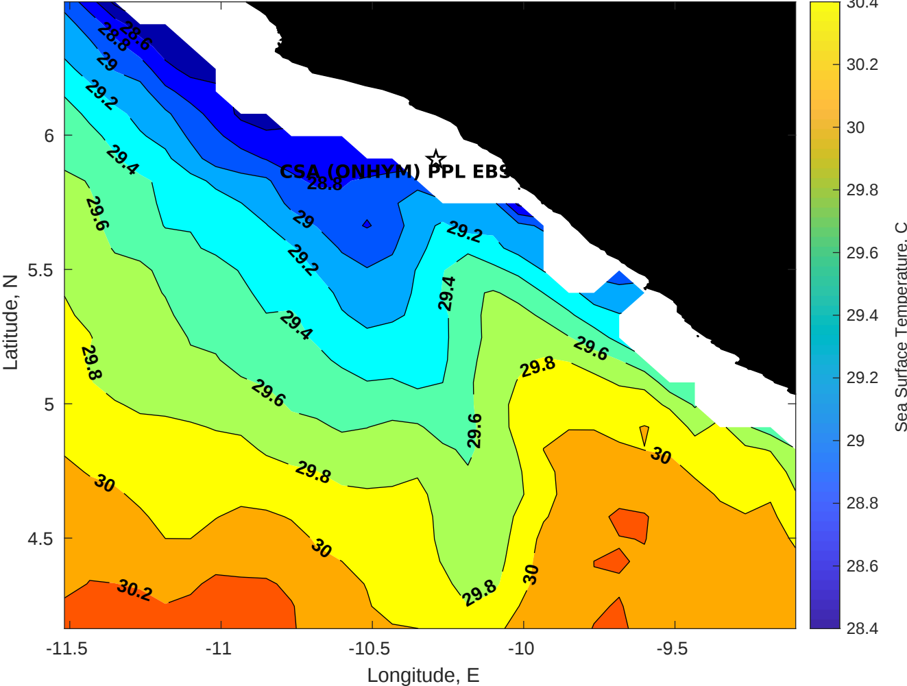
SST for CSA (ONHYM) PPL EBS - Liberia at 19-Apr-2025 00:00:00
