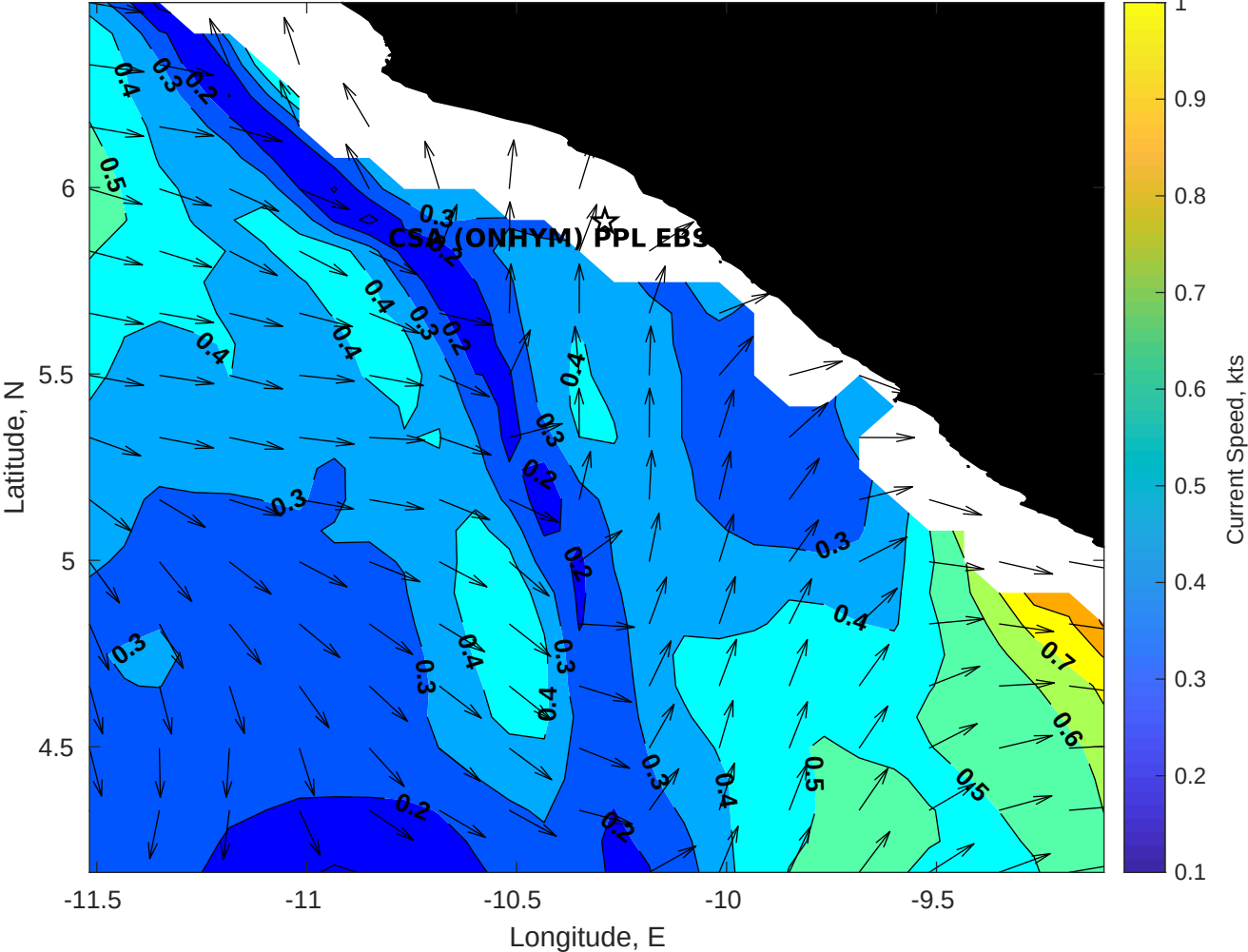
Surface Currents for CSA (ONHYM) PPL EBS - Liberia at 19-Apr-2025 00:00:00
