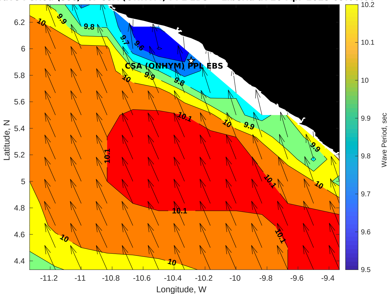
Wave Period (sec) for CSA (ONHYM) PPL EBS - Liberia at 20-Apr-2025 09:00:00
