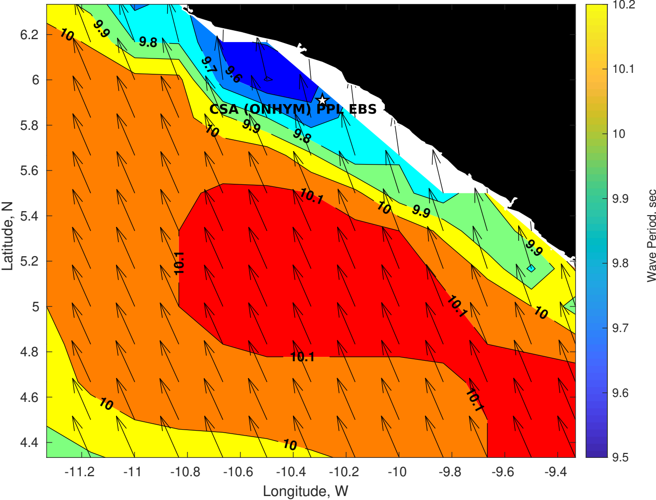
Wave Period (sec) for CSA (ONHYM) PPL EBS - Liberia at 20-Apr-2025 09:00:00
