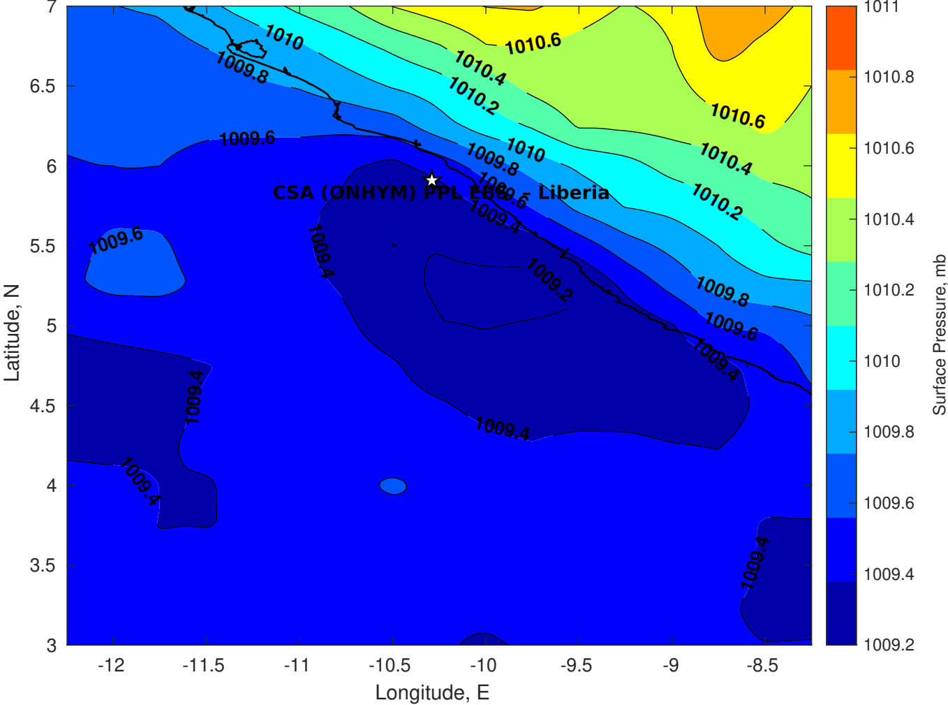
Surface Pressure (mb) for CSA (ONHYM) PPL EBS - Liberia at 21-Apr-2025 00:00:00
