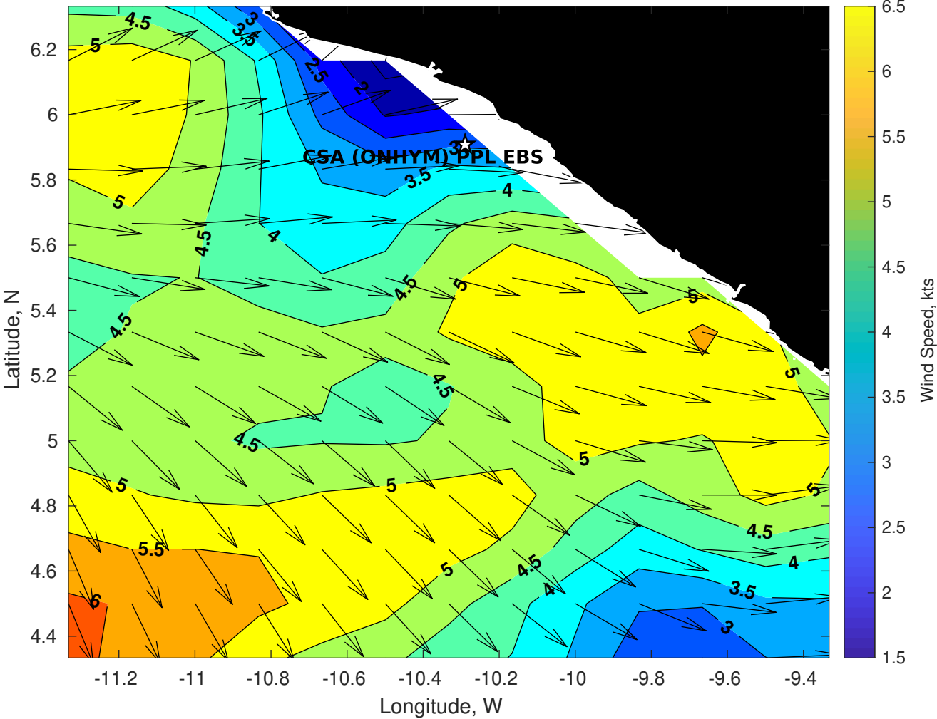
Winds (kts) for CSA (ONHYM) PPL EBS - Liberia at 20-Apr-2025 09:00:00
