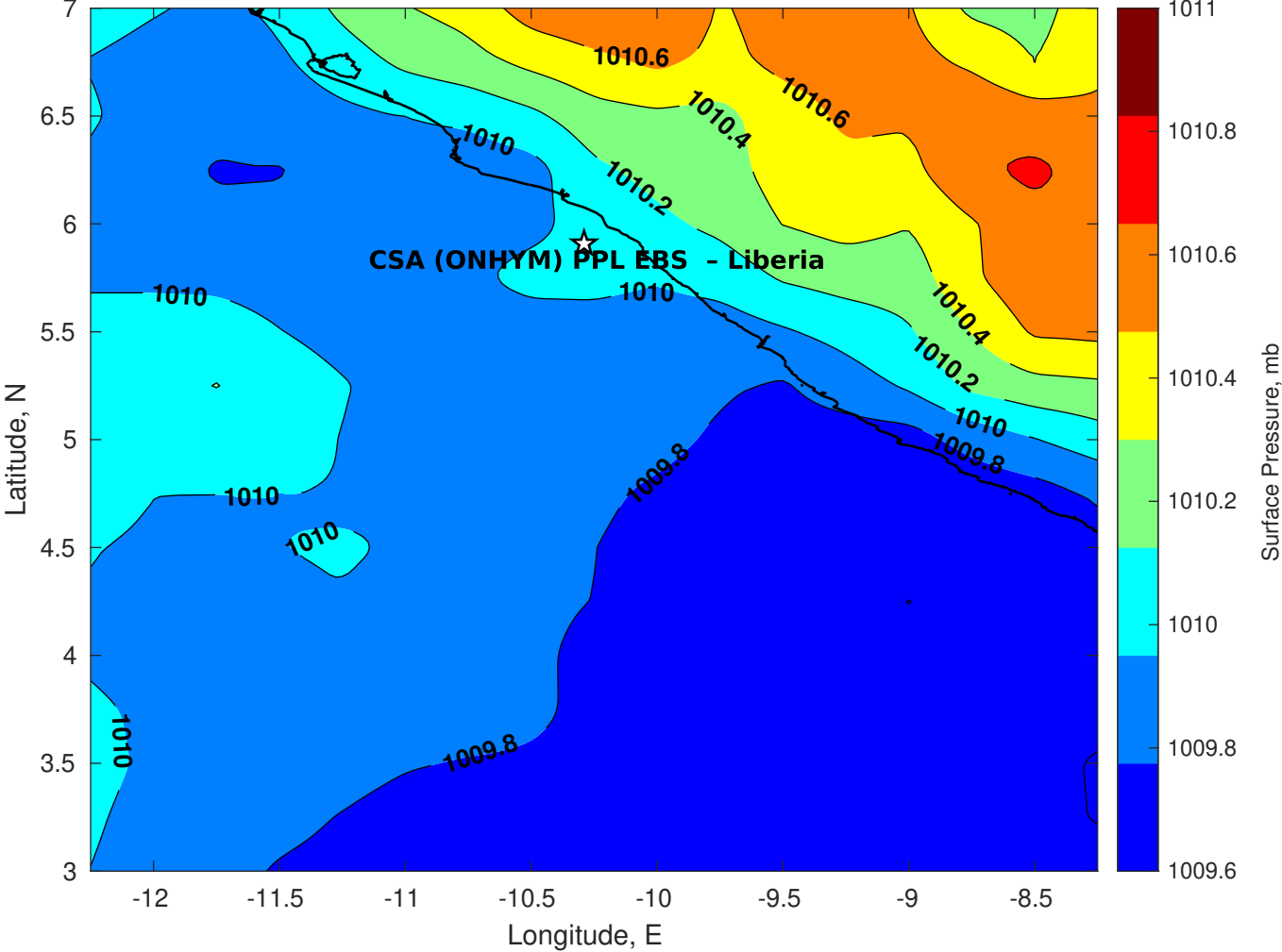
Surface Pressure (mb) for CSA (ONHYM) PPL EBS - Liberia at 22-Apr-2025 00:00:00
