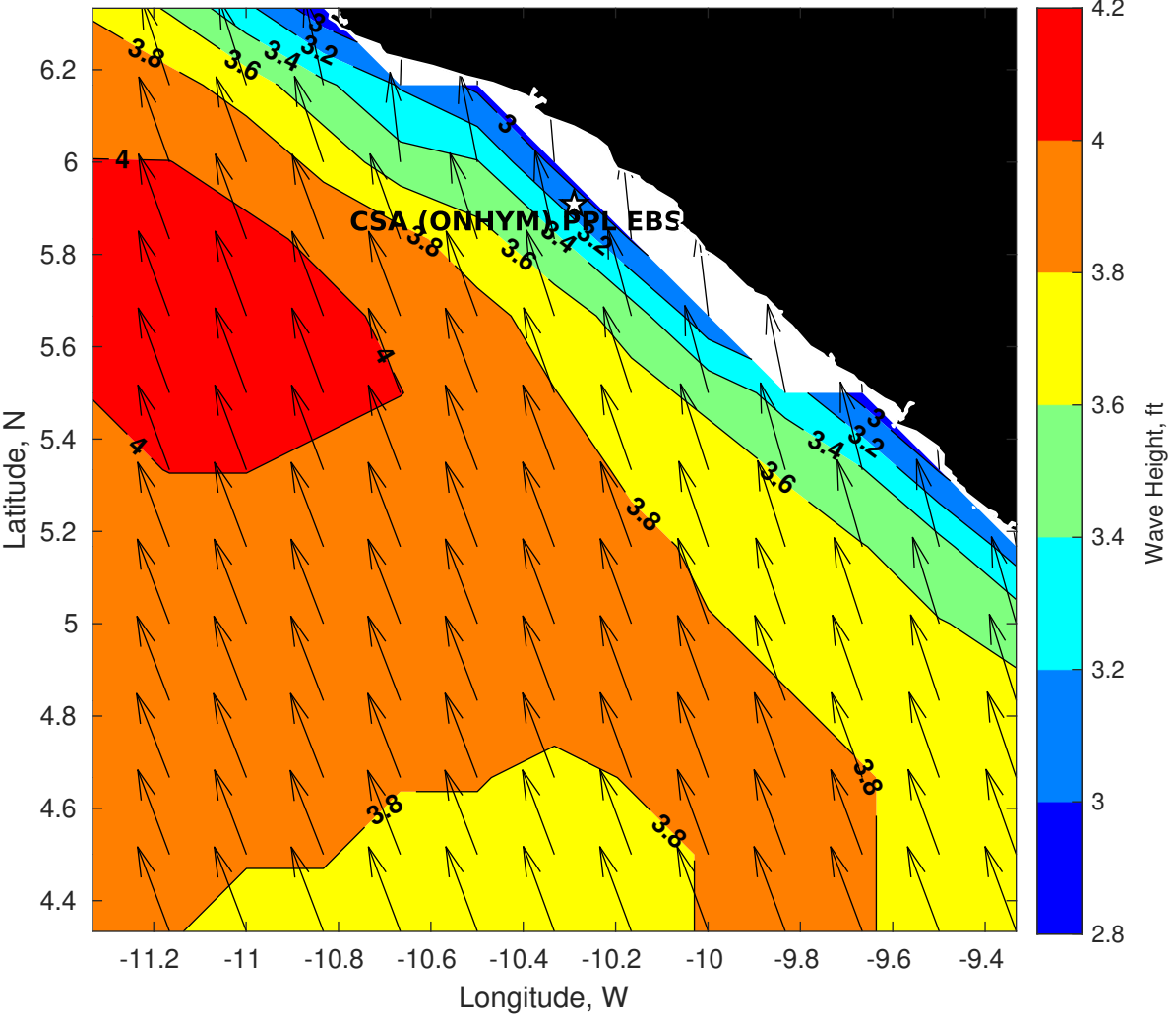
Wave Height (ft) for CSA (ONHYM) PPL EBS - Liberia at 20-Apr-2025 09:00:00
