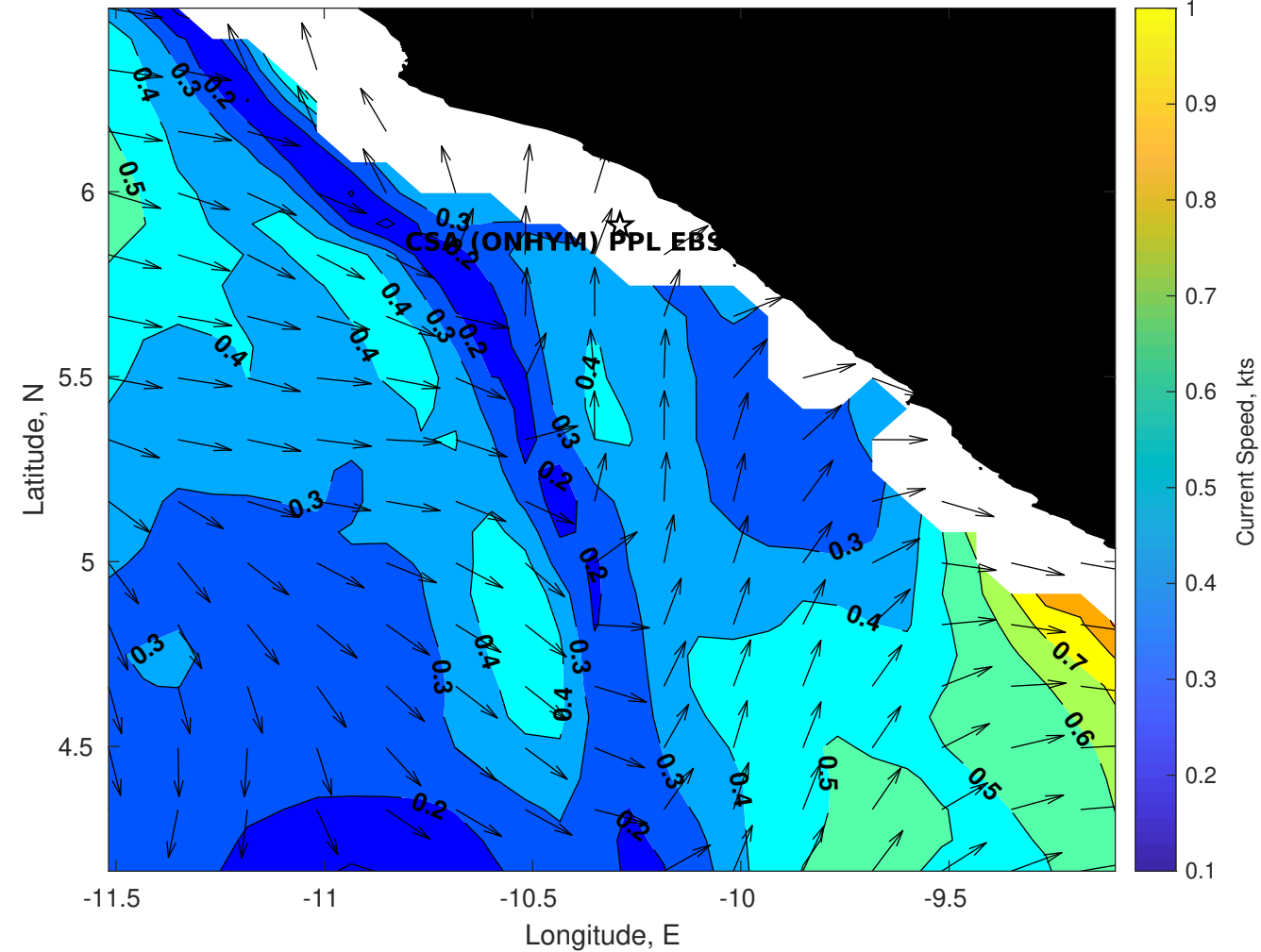
Surface Currents for CSA (ONHYM) PPL EBS - Liberia at 19-Apr-2025 00:00:00
