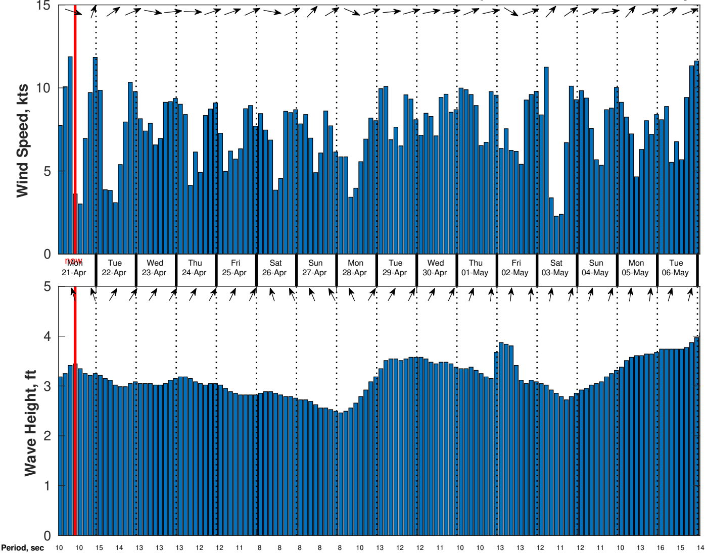
Wind & Wave Forecast for CSA (ONHYM) PPL EBS - Liberia from 20-Apr-2025 01:00:00 to 06-May-2025 01:00:00
