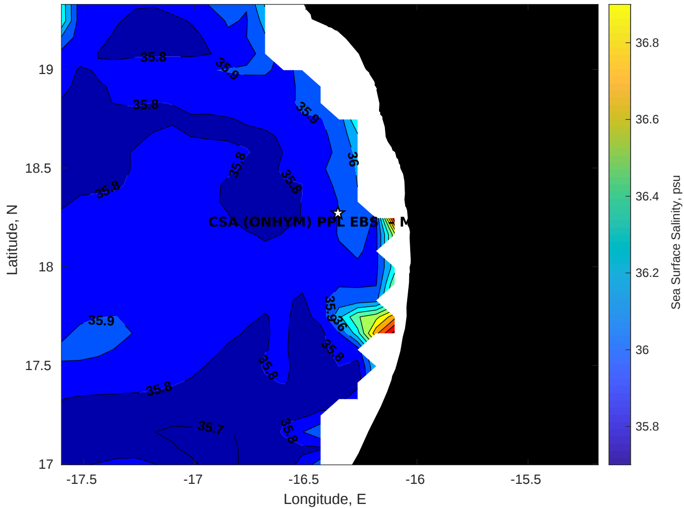
Surface Salinity for CSA (ONHYM) PPL EBS - Mauritania at 19-Apr-2025 00:00:00
