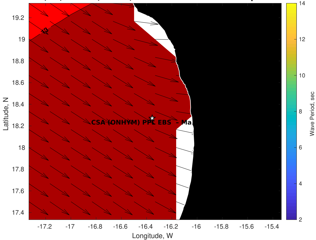
Wave Period (sec) for CSA (ONHYM) PPL EBS - Mauritania at 20-Apr-2025 09:00:00
