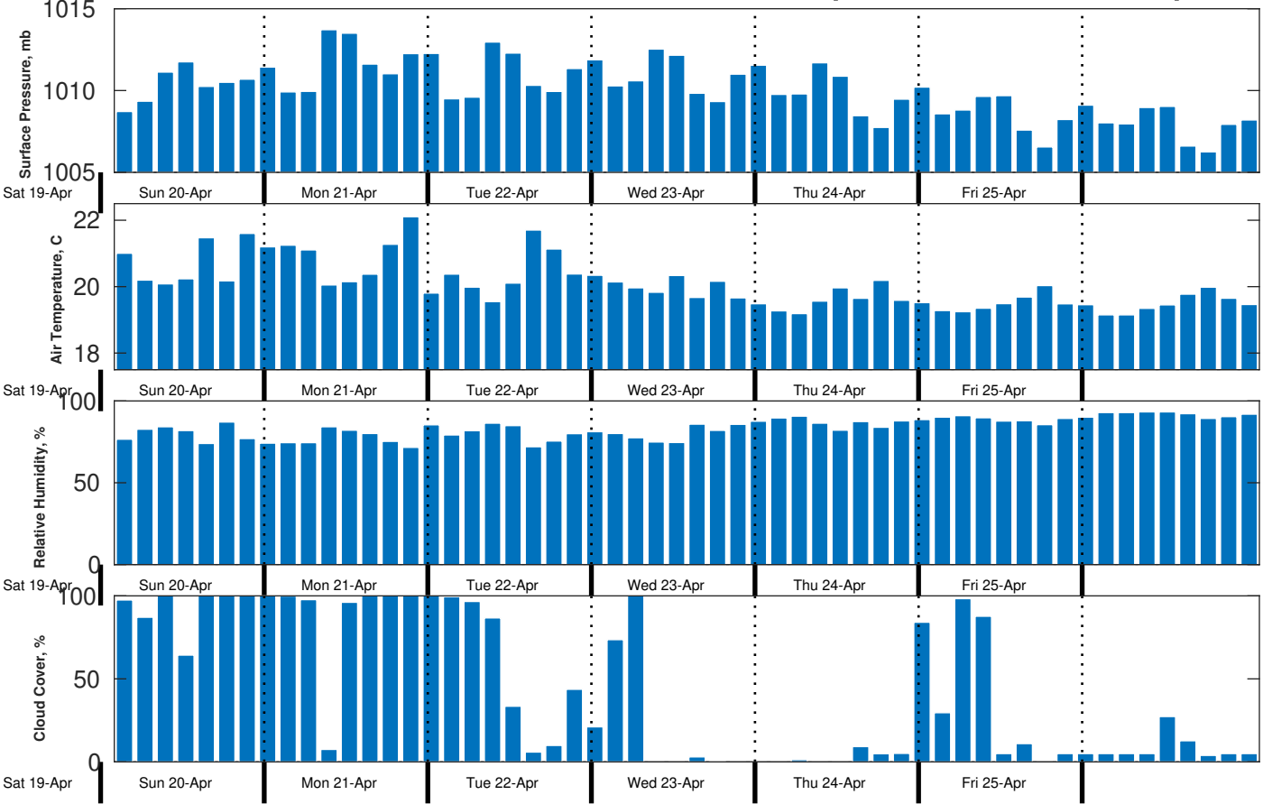
Met Forecast for CSA (ONHYM) PPL EBS - Mauritania from 20-Apr-2025 00:00:00 to 27-Apr-2025 00:00:00
