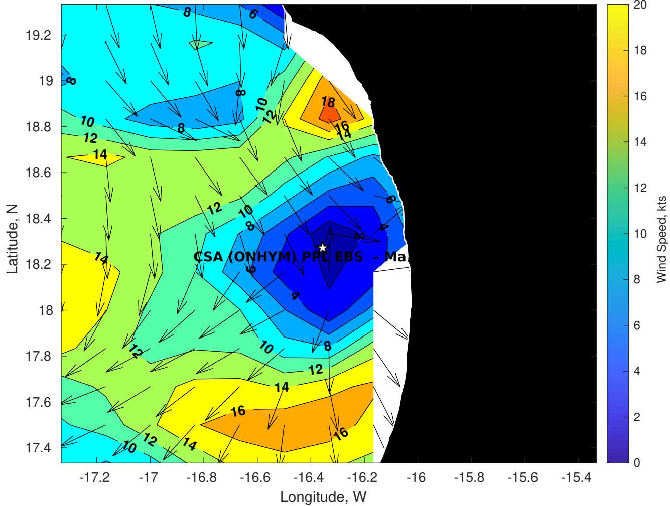
Winds (kts) for CSA (ONHYM) PPL EBS - Mauritania at 20-Apr-2025 09:00:00
