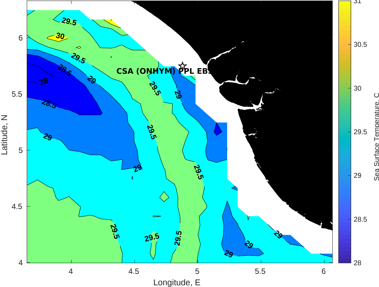
SST for CSA (ONHYM) PPL EBS - Nigeria at 19-Apr-2025 00:00:00
