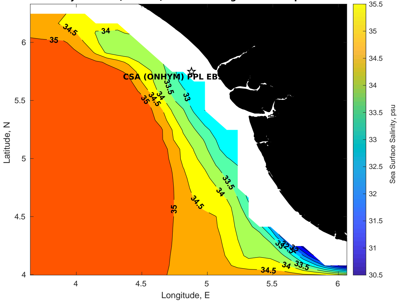
Surface Salinity for CSA (ONHYM) PPL EBS - Nigeria at 19-Apr-2025 00:00:00
