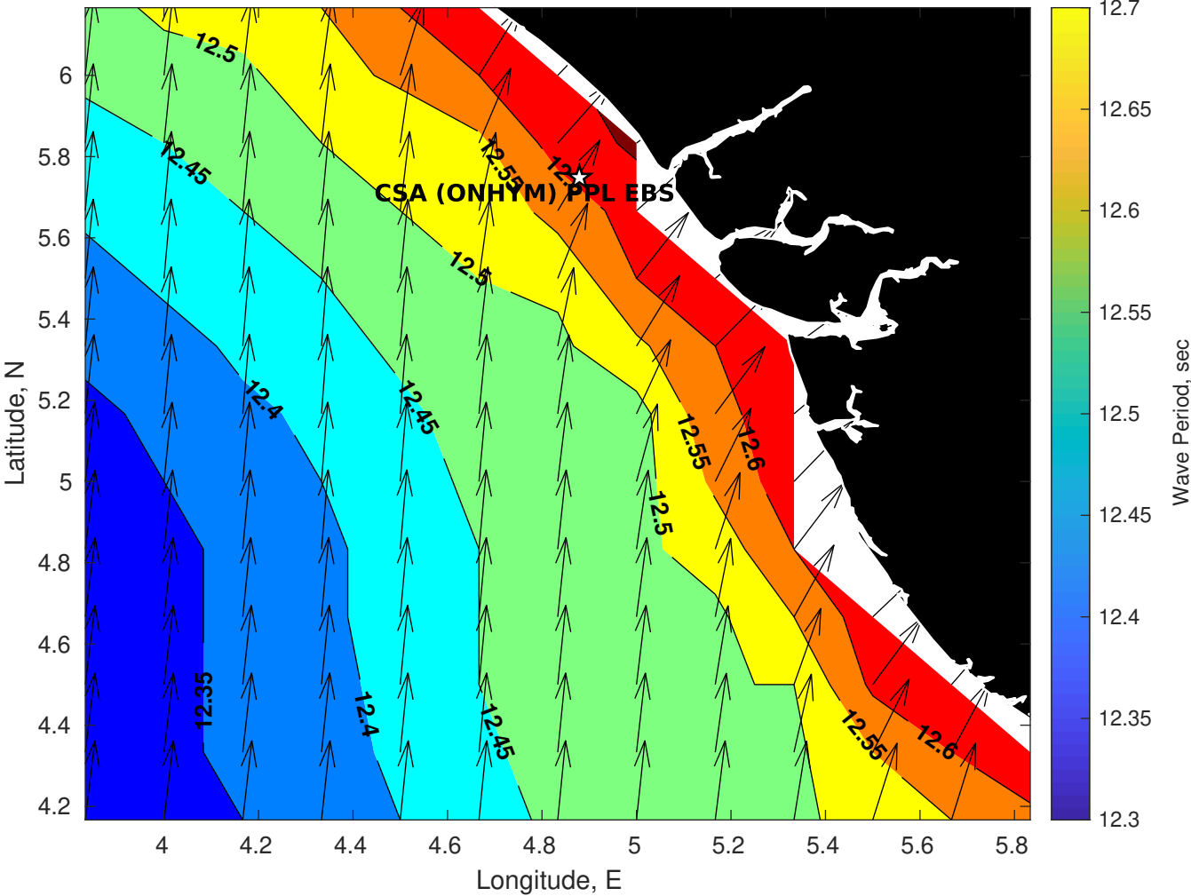
Wave Period (sec) for CSA (ONHYM) PPL EBS - Nigeria at 20-Apr-2025 09:00:00
