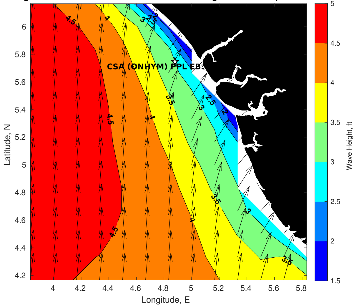
Wave Height (ft) for CSA (ONHYM) PPL EBS - Nigeria at 20-Apr-2025 09:00:00
