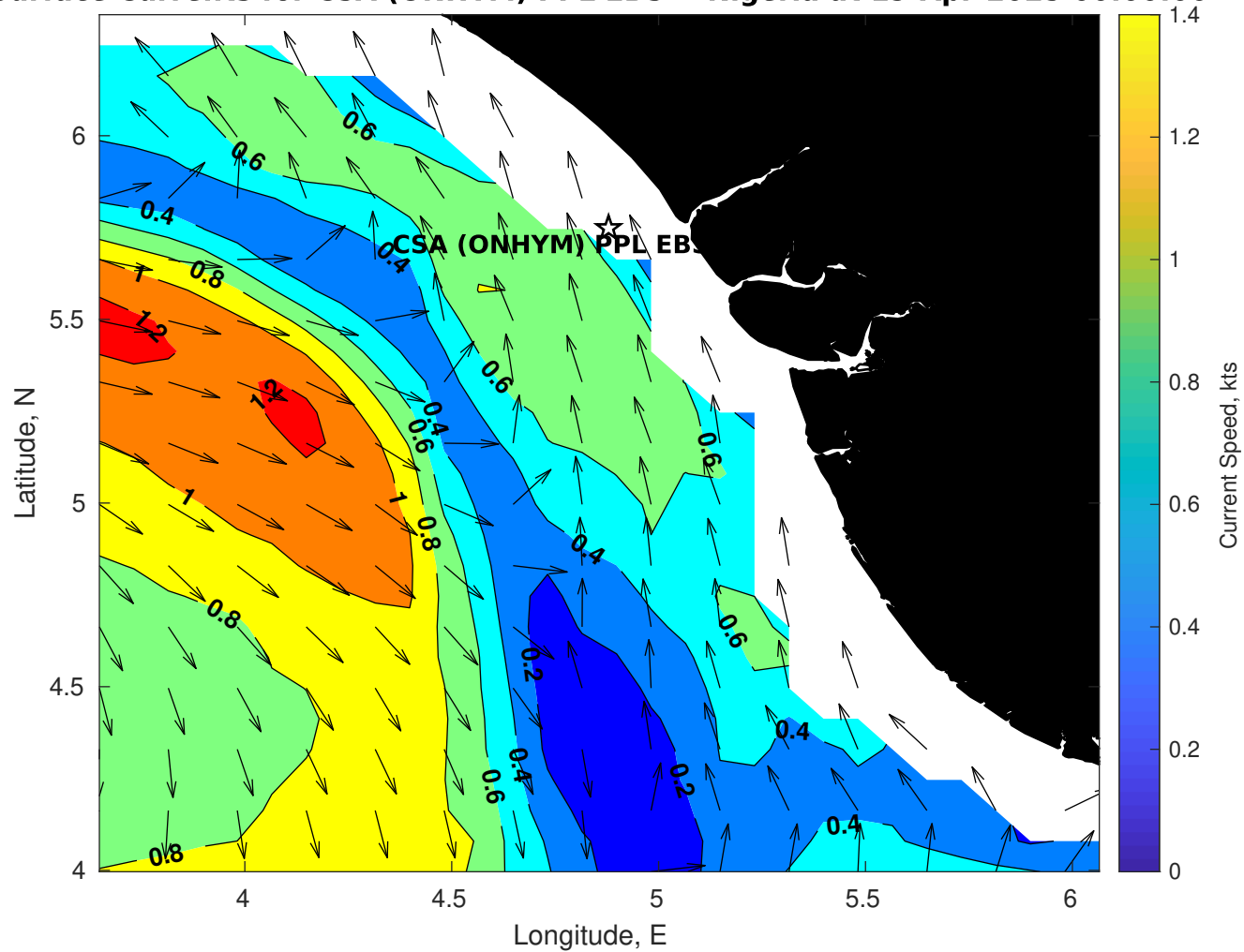
Surface Currents for CSA (ONHYM) PPL EBS - Nigeria at 19-Apr-2025 00:00:00
