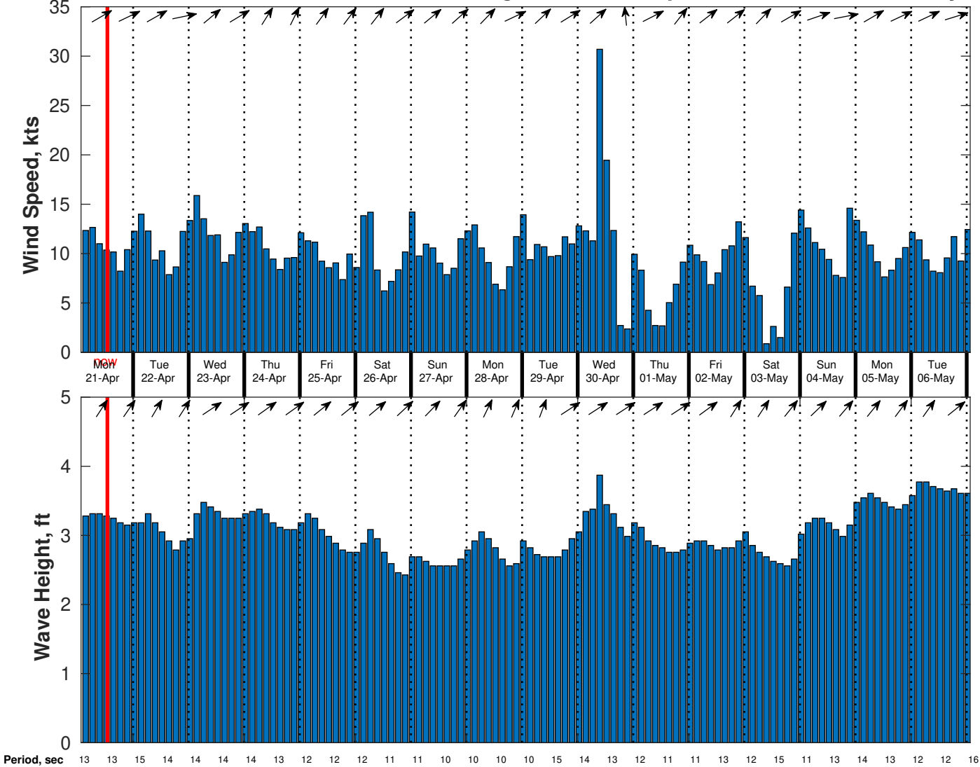
Wind & Wave Forecast for CSA (ONHYM) PPL EBS - Nigeria from 20-Apr-2025 02:00:00 to 06-May-2025 02:00:00
