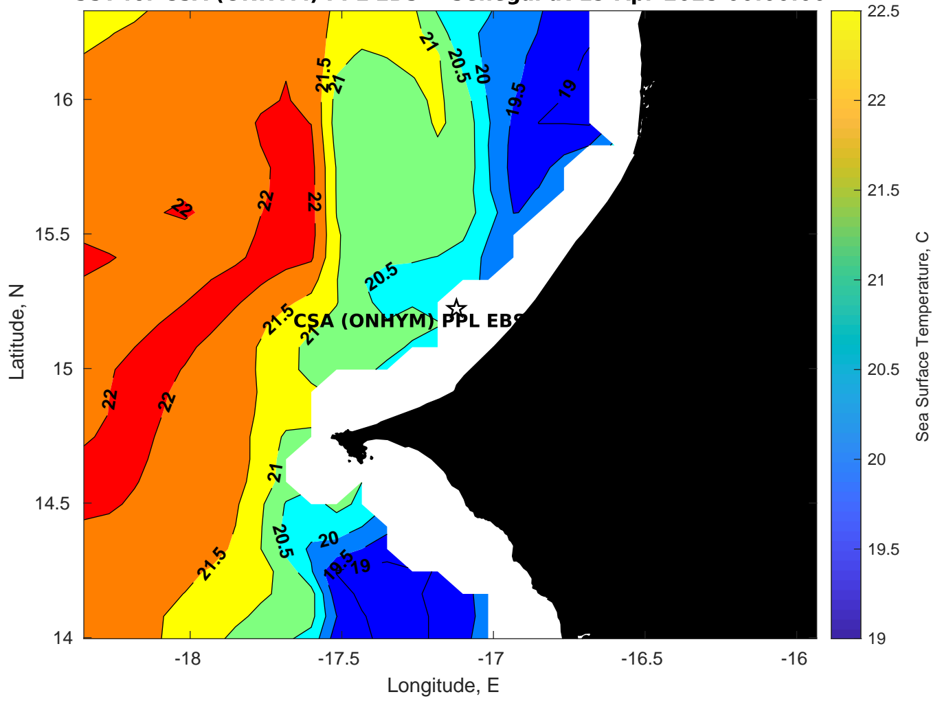
SST for CSA (ONHYM) PPL EBS - Senegal at 19-Apr-2025 00:00:00
