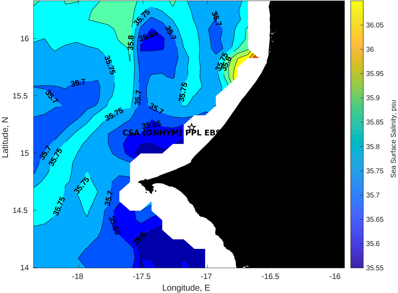
Surface Salinity for CSA (ONHYM) PPL EBS - Senegal at 19-Apr-2025 00:00:00
