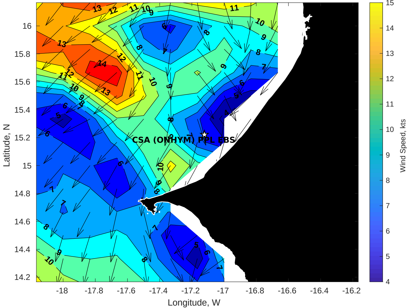
Winds (kts) for CSA (ONHYM) PPL EBS - Senegal at 20-Apr-2025 09:00:00
