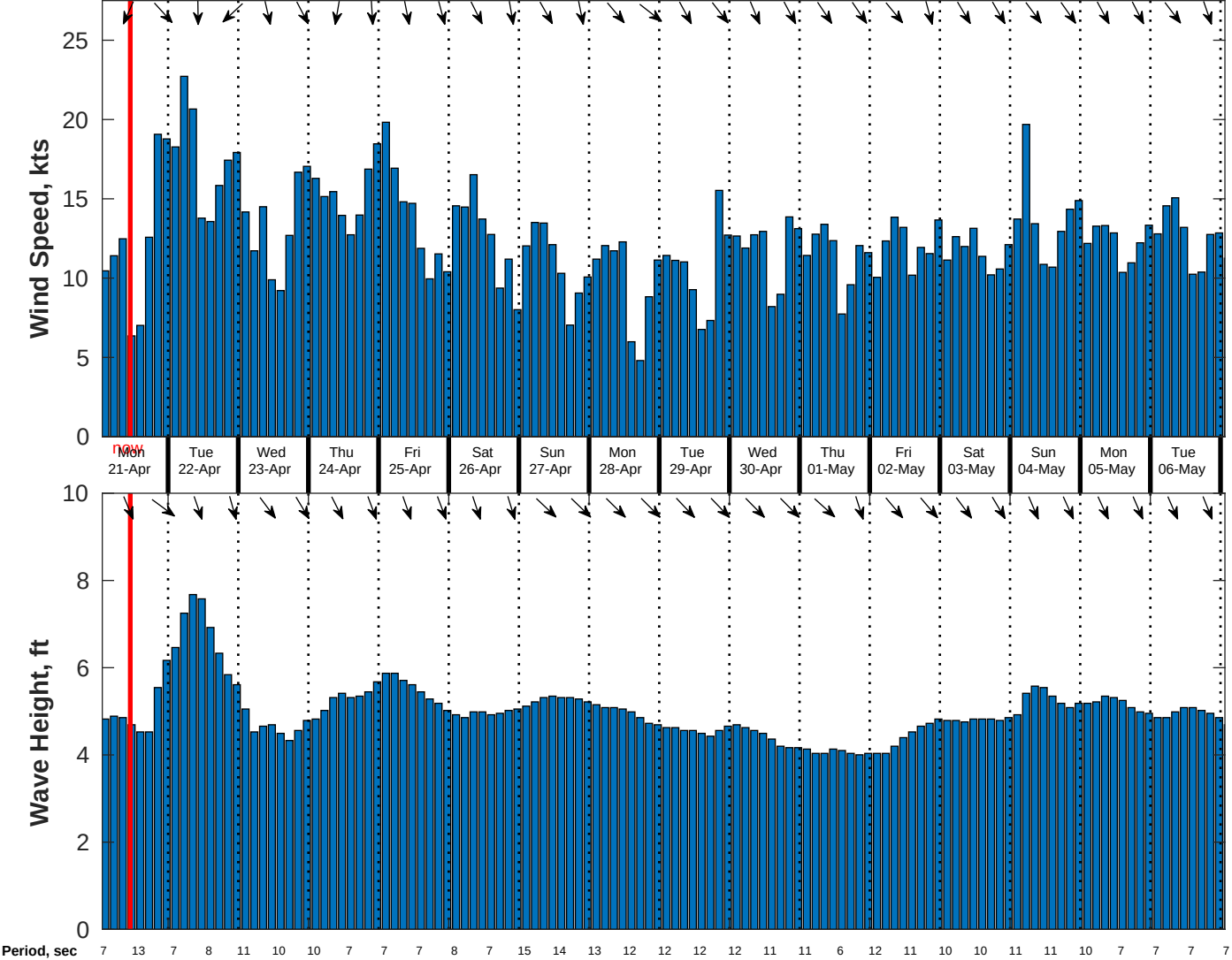
Wind & Wave Forecast for CSA (ONHYM) PPL EBS - Senegal from 20-Apr-2025 01:00:00 to 06-May-2025 01:00:00
