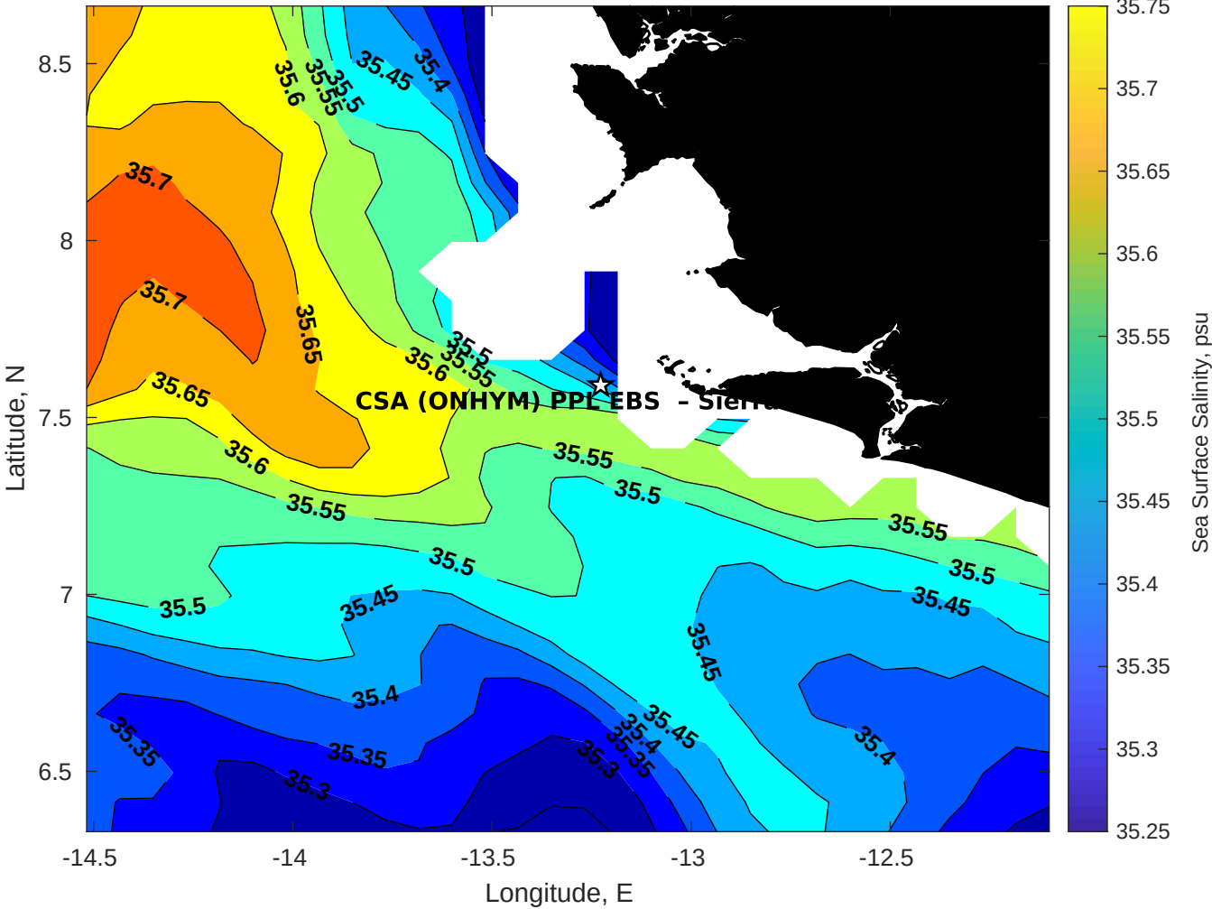
Surface Salinity for CSA (ONHYM) PPL EBS - Sierra Leone at 19-Apr-2025 00:00:00
