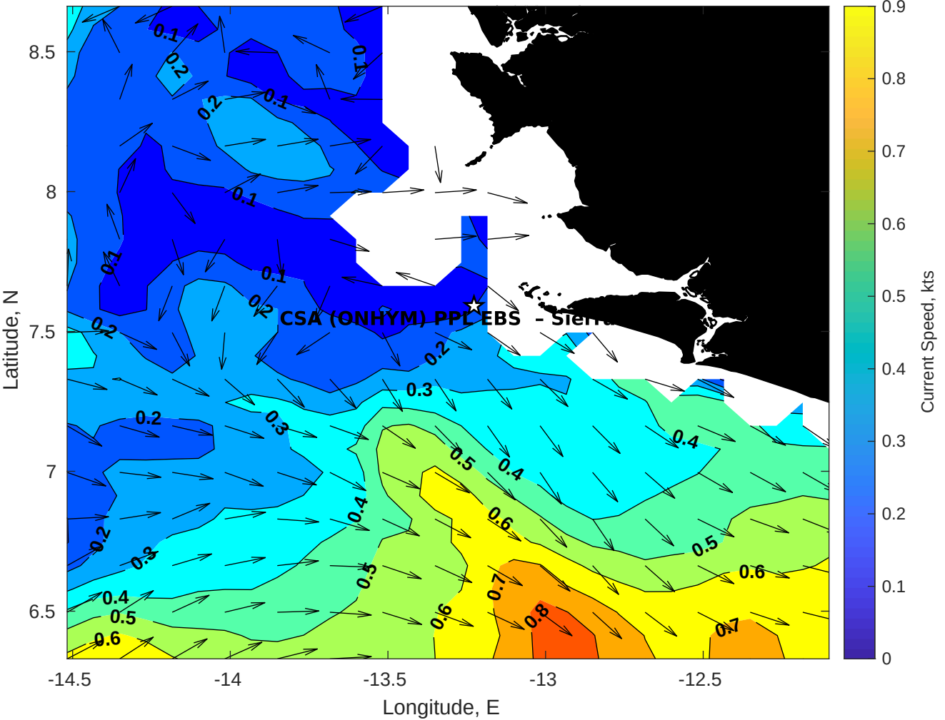
Surface Currents for CSA (ONHYM) PPL EBS - Sierra Leone at 19-Apr-2025 00:00:00
