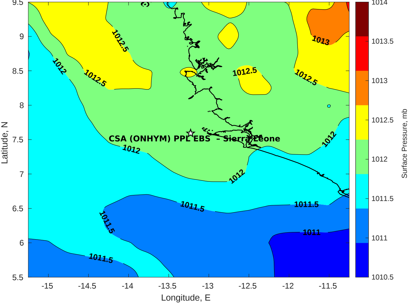
Surface Pressure (mb) for CSA (ONHYM) PPL EBS - Sierra Leone at 20-Apr-2025 00:00:00
