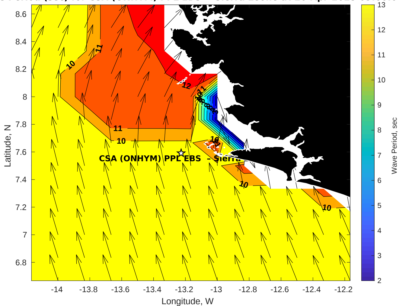
Wave Period (sec) for CSA (ONHYM) PPL EBS - Sierra Leone at 20-Apr-2025 09:00:00
