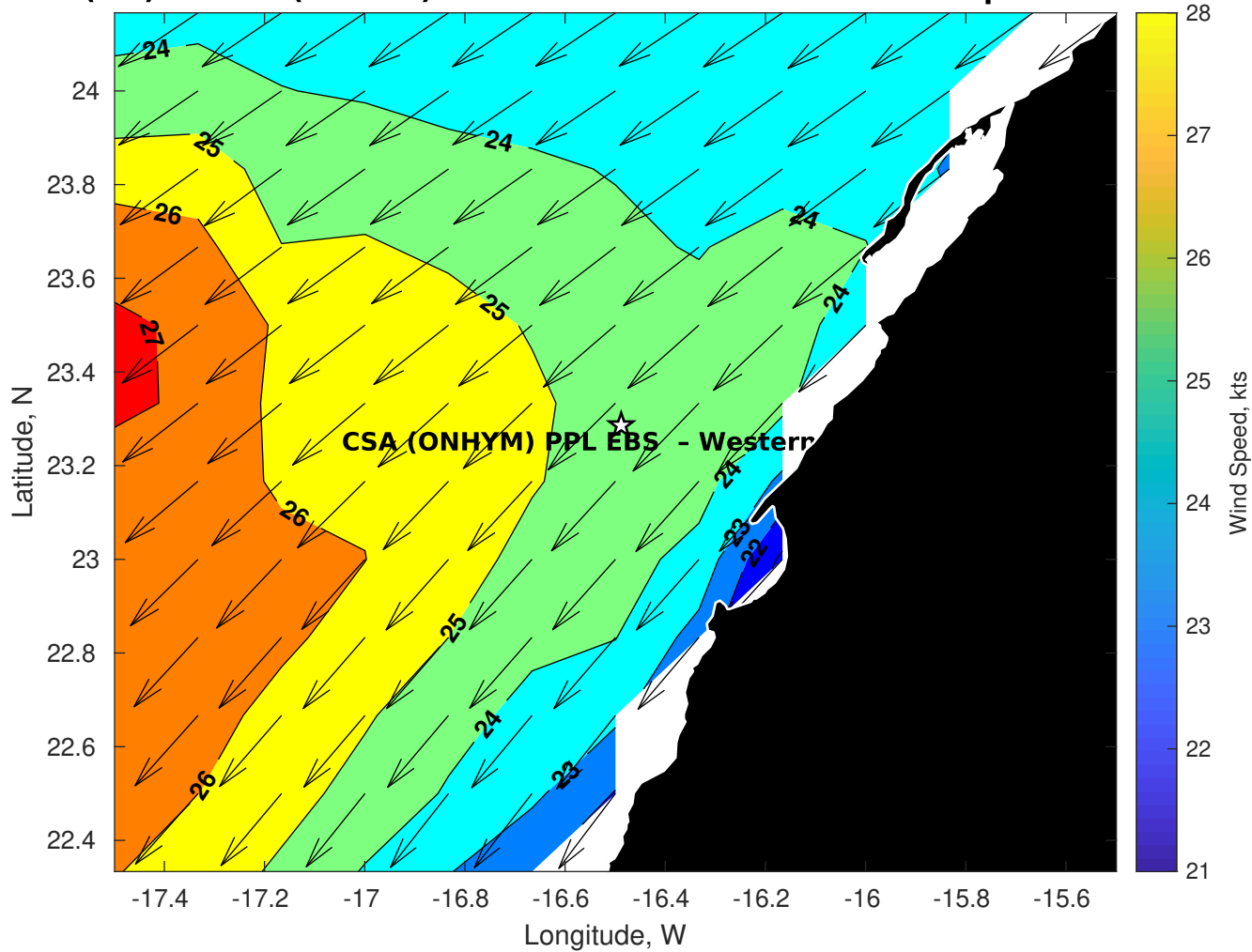
Winds (kts) for CSA (ONHYM) PPL EBS - Western Sahara at 20-Apr-2025 09:00:00
