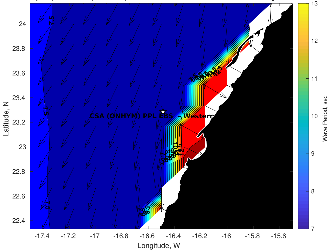
Wave Period (sec) for CSA (ONHYM) PPL EBS - Western Sahara at 20-Apr-2025 09:00:00
