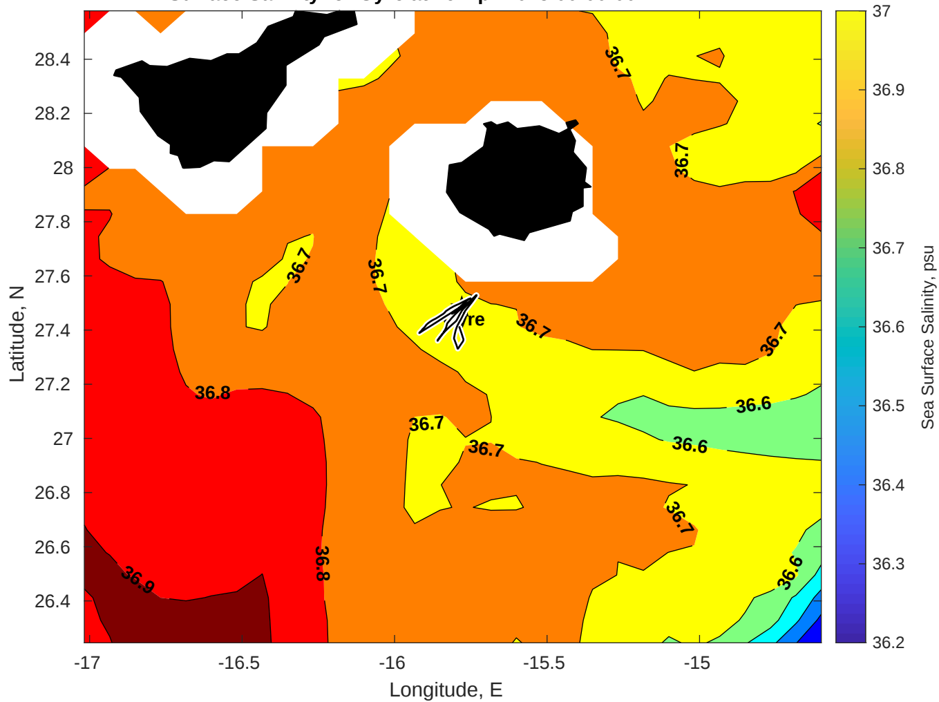
Surface Salinity for Gyre at 19-Apr-2025 00:00:00
