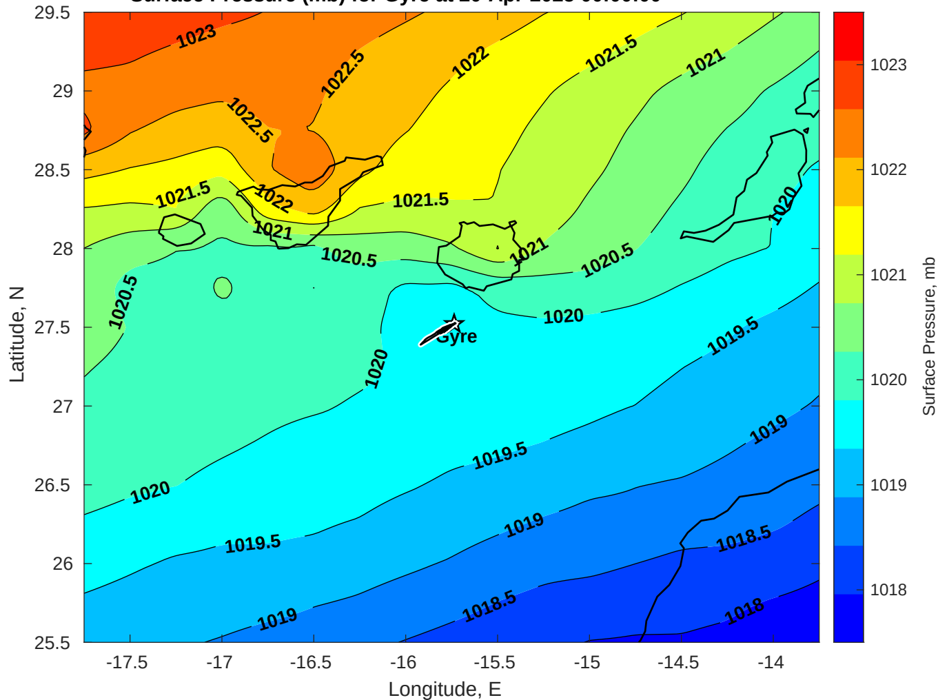
Surface Pressure (mb) for Gyre at 20-Apr-2025 00:00:00
