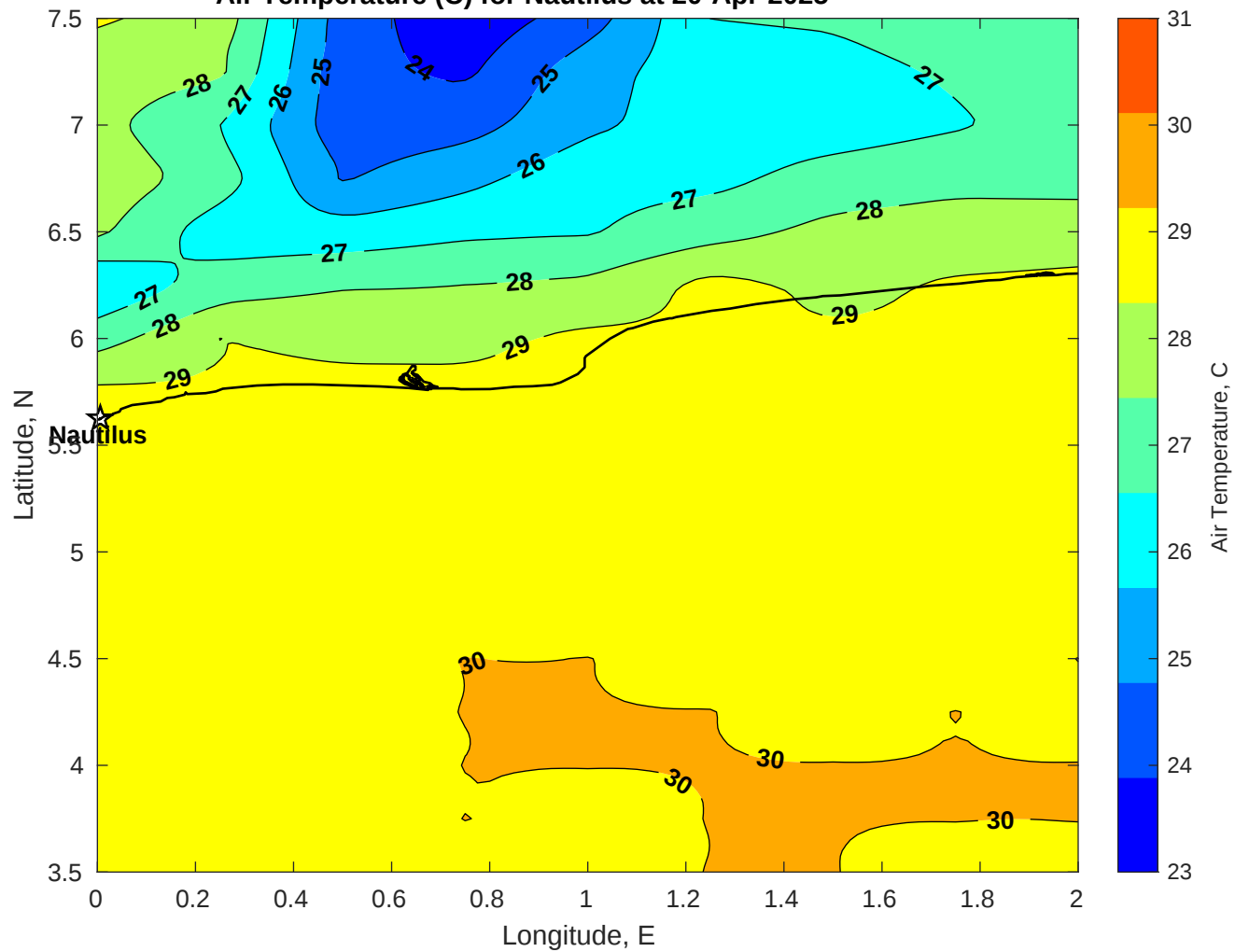
Air Temperature (C) for Nautilus at 20-Apr-2025
