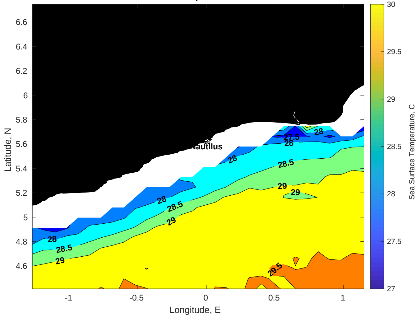
SST for Nautilus at 19-Apr-2025 00:00:00
