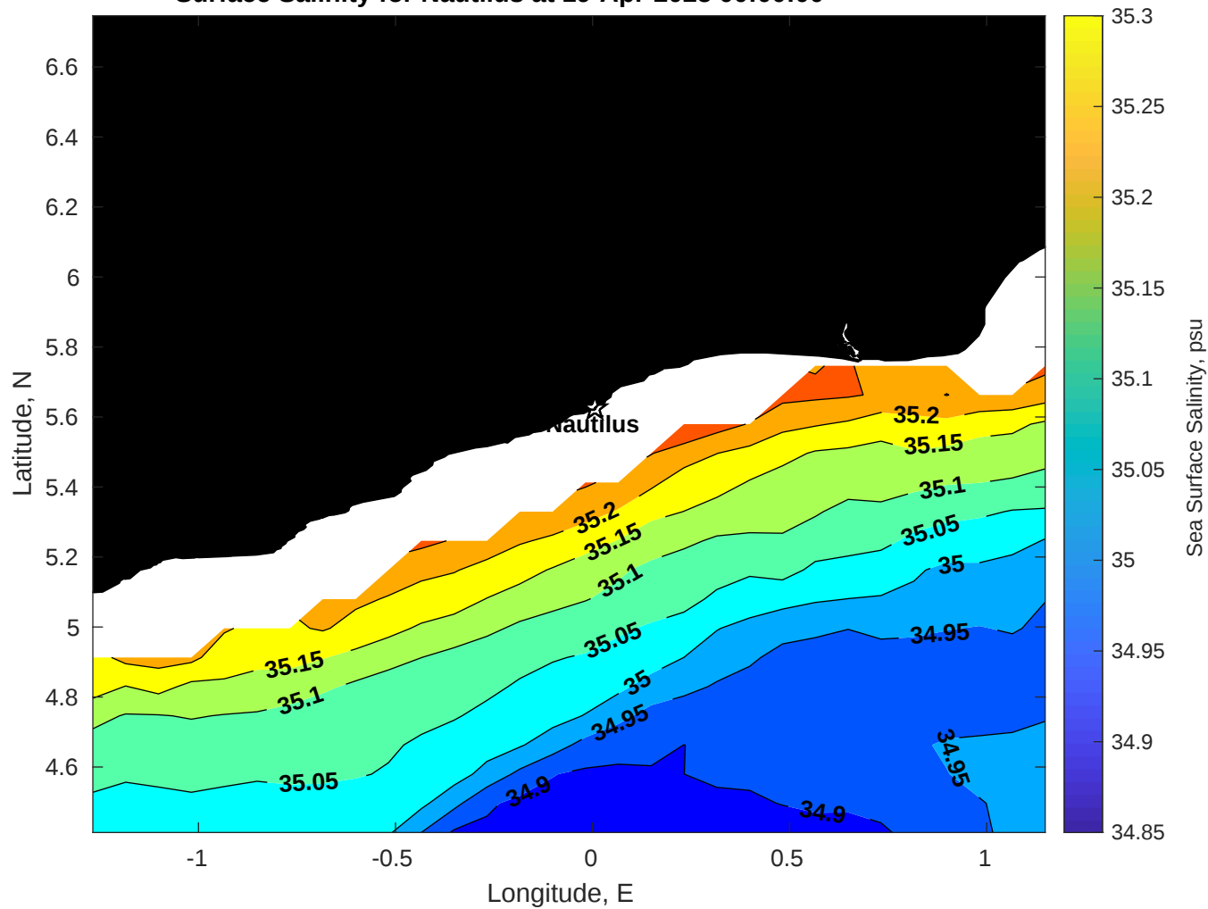
Surface Salinity for Nautilus at 19-Apr-2025 00:00:00
