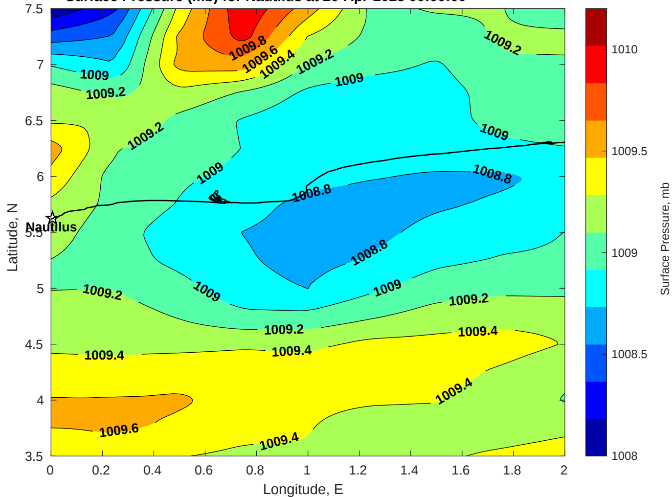
Surface Pressure (mb) for Nautilus at 20-Apr-2025 00:00:00
