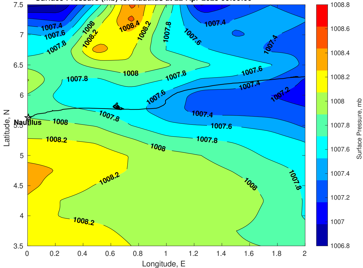
Surface Pressure (mb) for Nautilus at 22-Apr-2025 00:00:00
