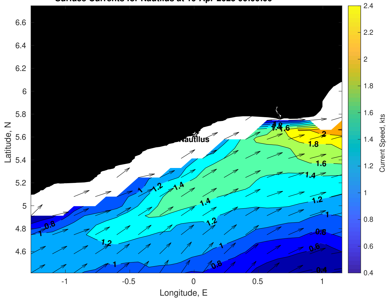
Surface Currents for Nautilus at 19-Apr-2025 00:00:00
