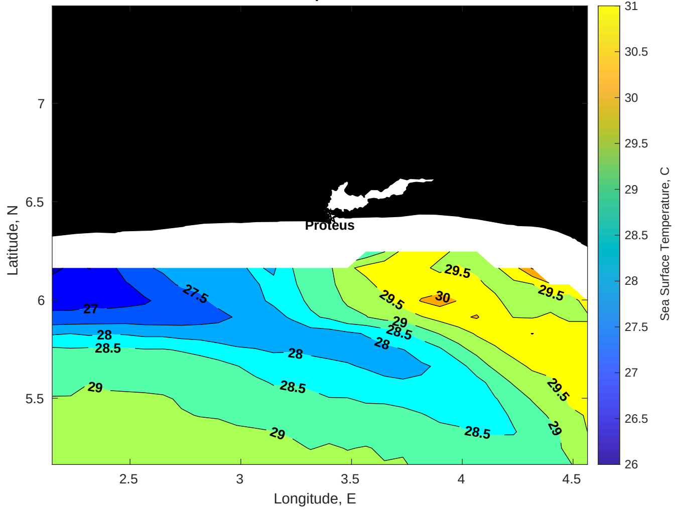
SST for Proteus at 19-Apr-2025 00:00:00
