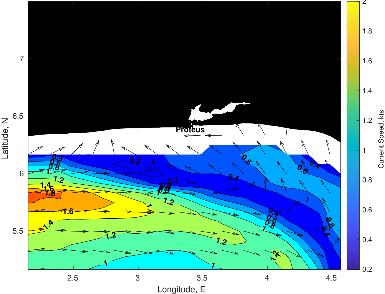
Surface Currents for Proteus at 19-Apr-2025 00:00:00
