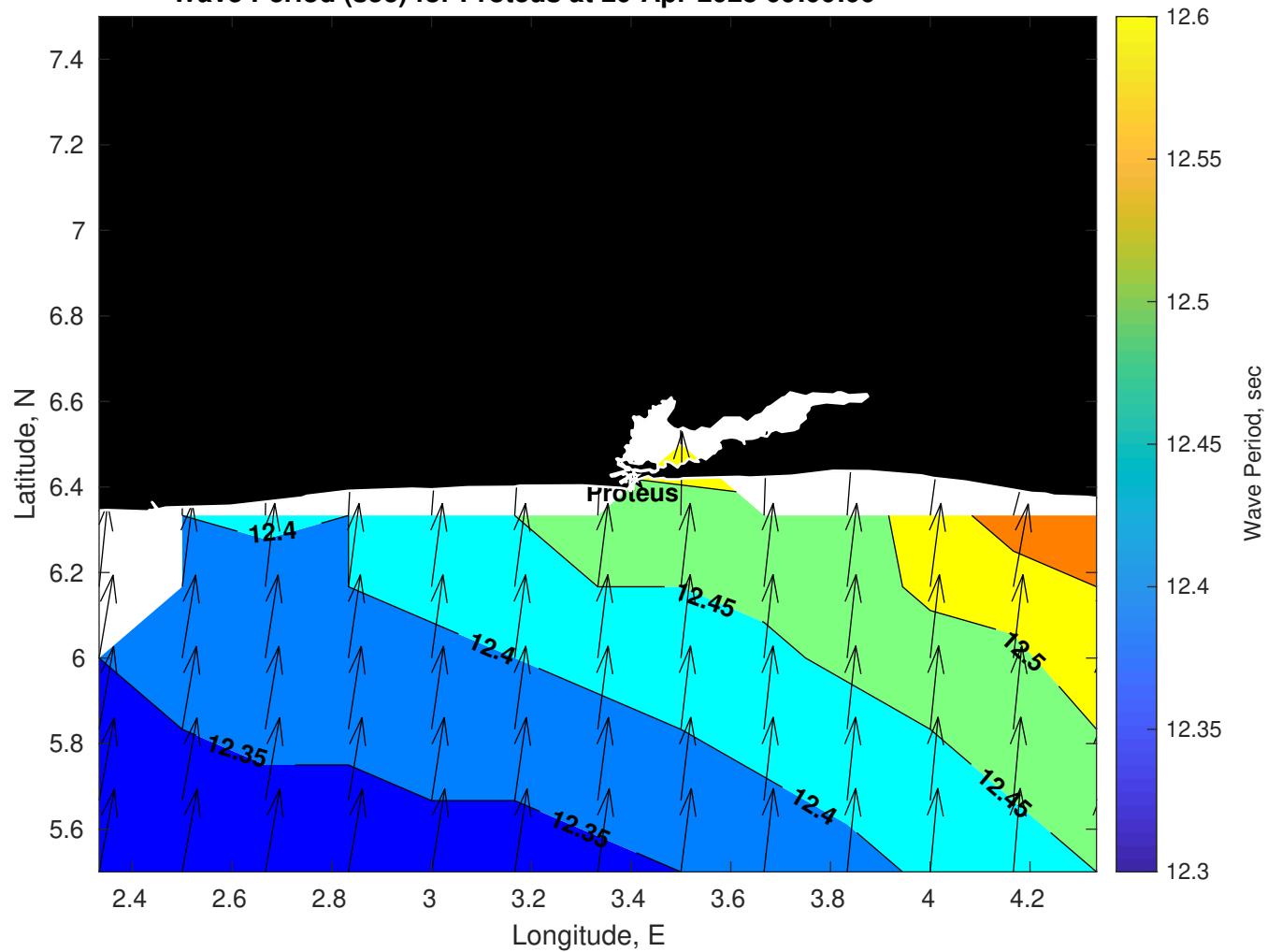
Wave Period (sec) for Proteus at 20-Apr-2025 09:00:00
