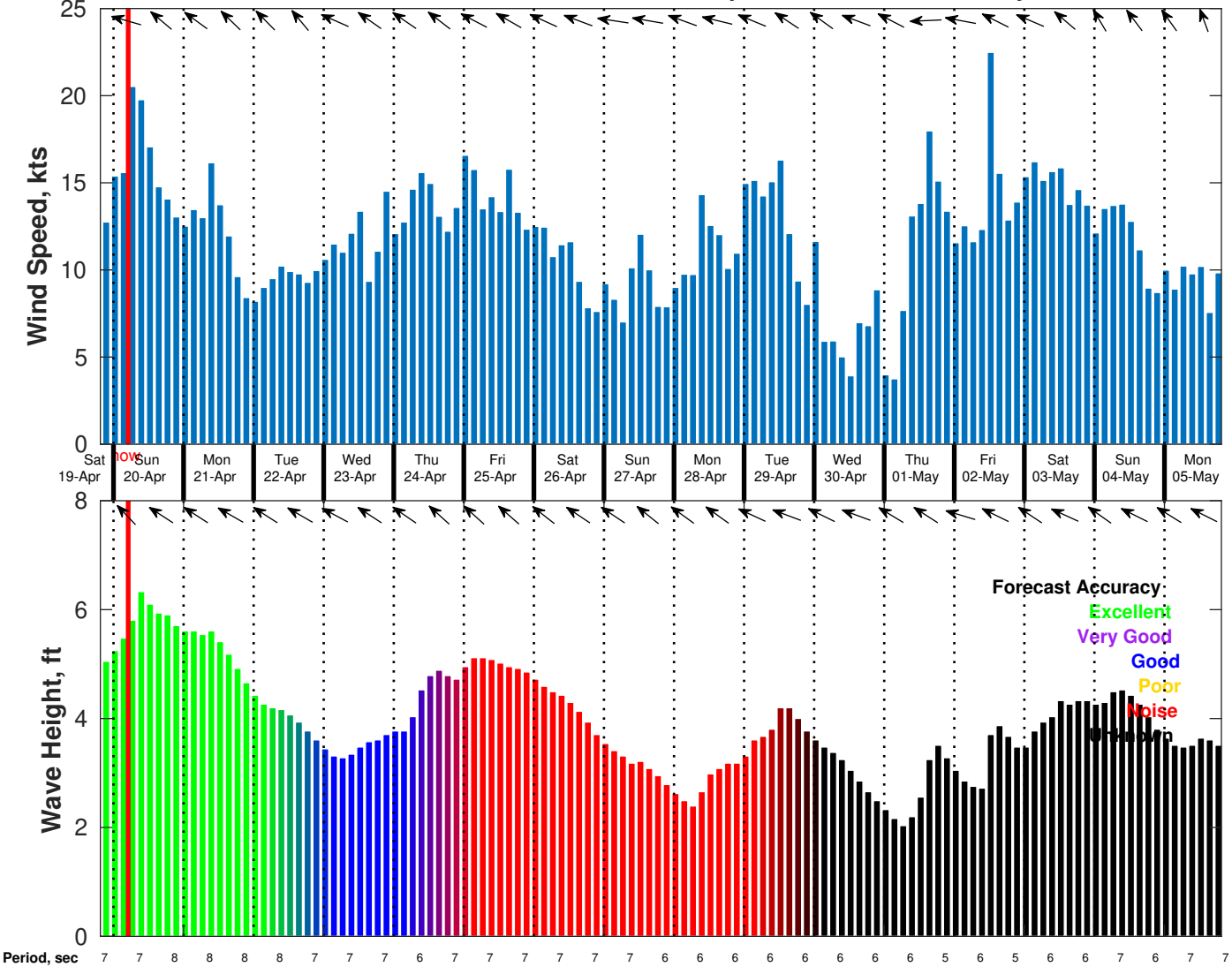
Wind & Wave Forecast for Shell Noches GC19 PPL Geotechnical from 19-Apr-2025 20:00:00 to 05-May-2025 20:00:00
