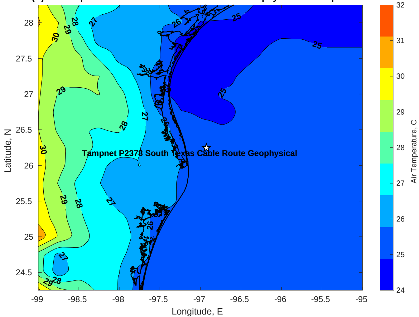
Air Temperature (C) for Tampnet P2378 South Texas Cable Route Geophysical at 20-Apr-2025
