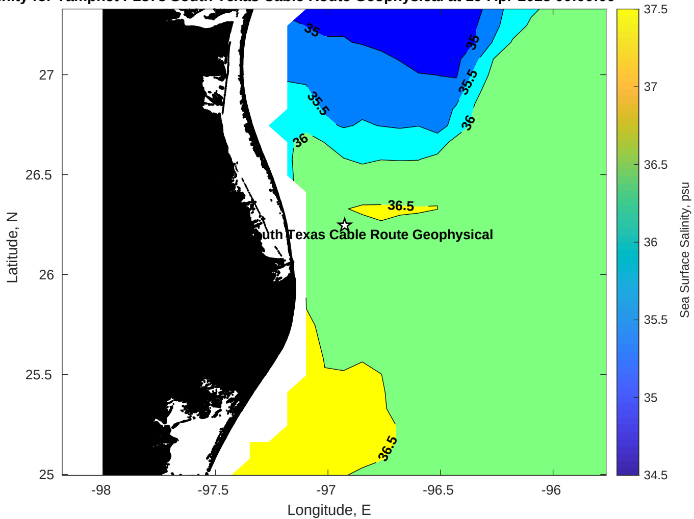
Surface Salinity for Tampnet P2378 South Texas Cable Route Geophysical at 19-Apr-2025 00:00:00
