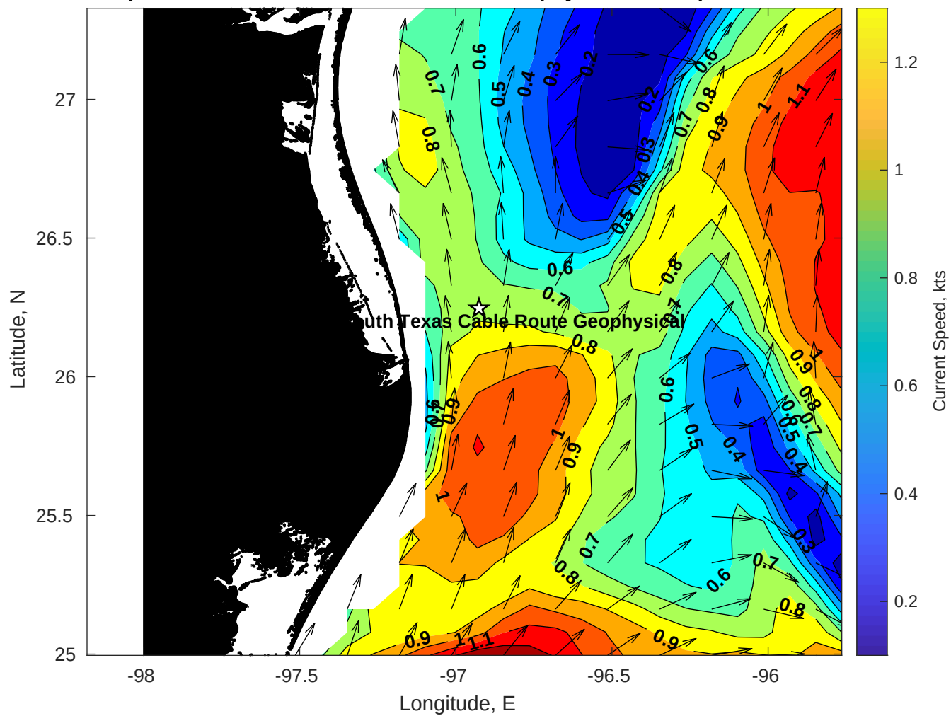
Surface Currents for Tampnet P2378 South Texas Cable Route Geophysical at 19-Apr-2025 00:00:00
