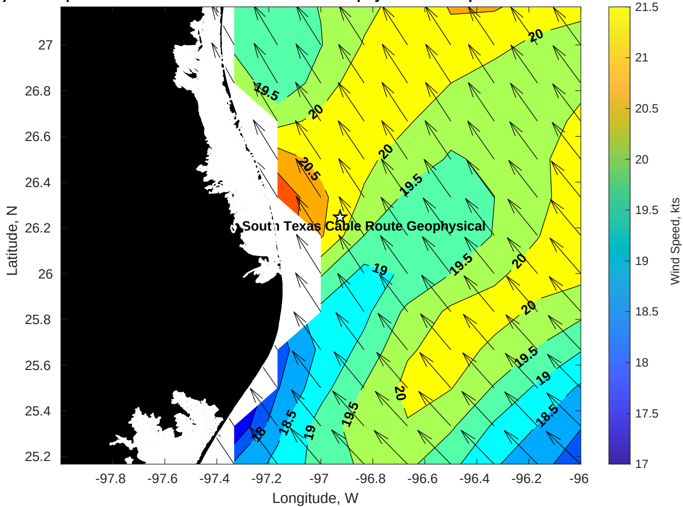
Winds (kts) for Tampnet P2378 South Texas Cable Route Geophysical at 20-Apr-2025 09:00:00
