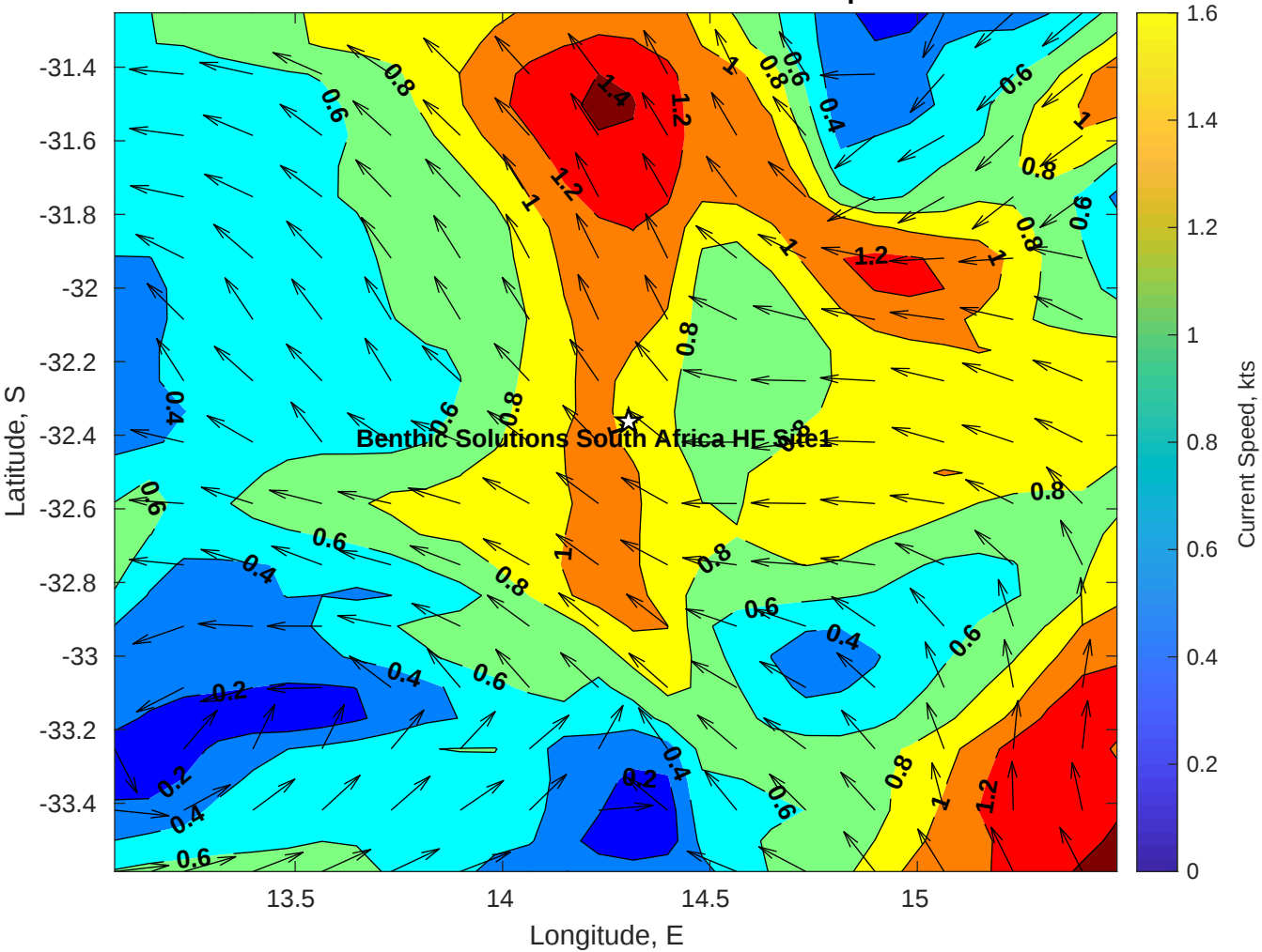
Surface Currents for Benthic Solutions South Africa HF Site1 at 20-Apr-2025 00:00:00
