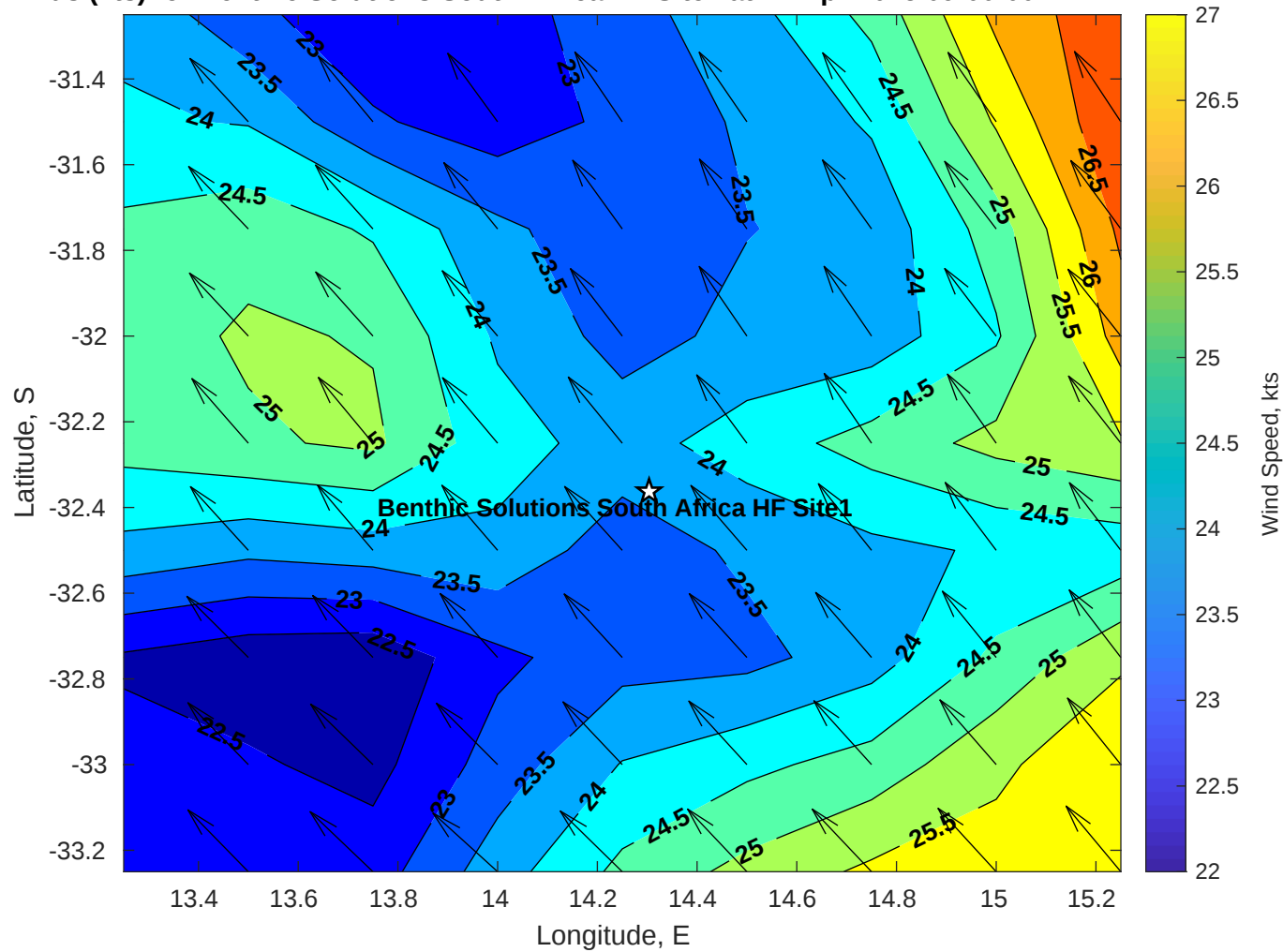
Winds (kts) for Benthic Solutions South Africa HF Site1 at 21-Apr-2025 09:00:00
