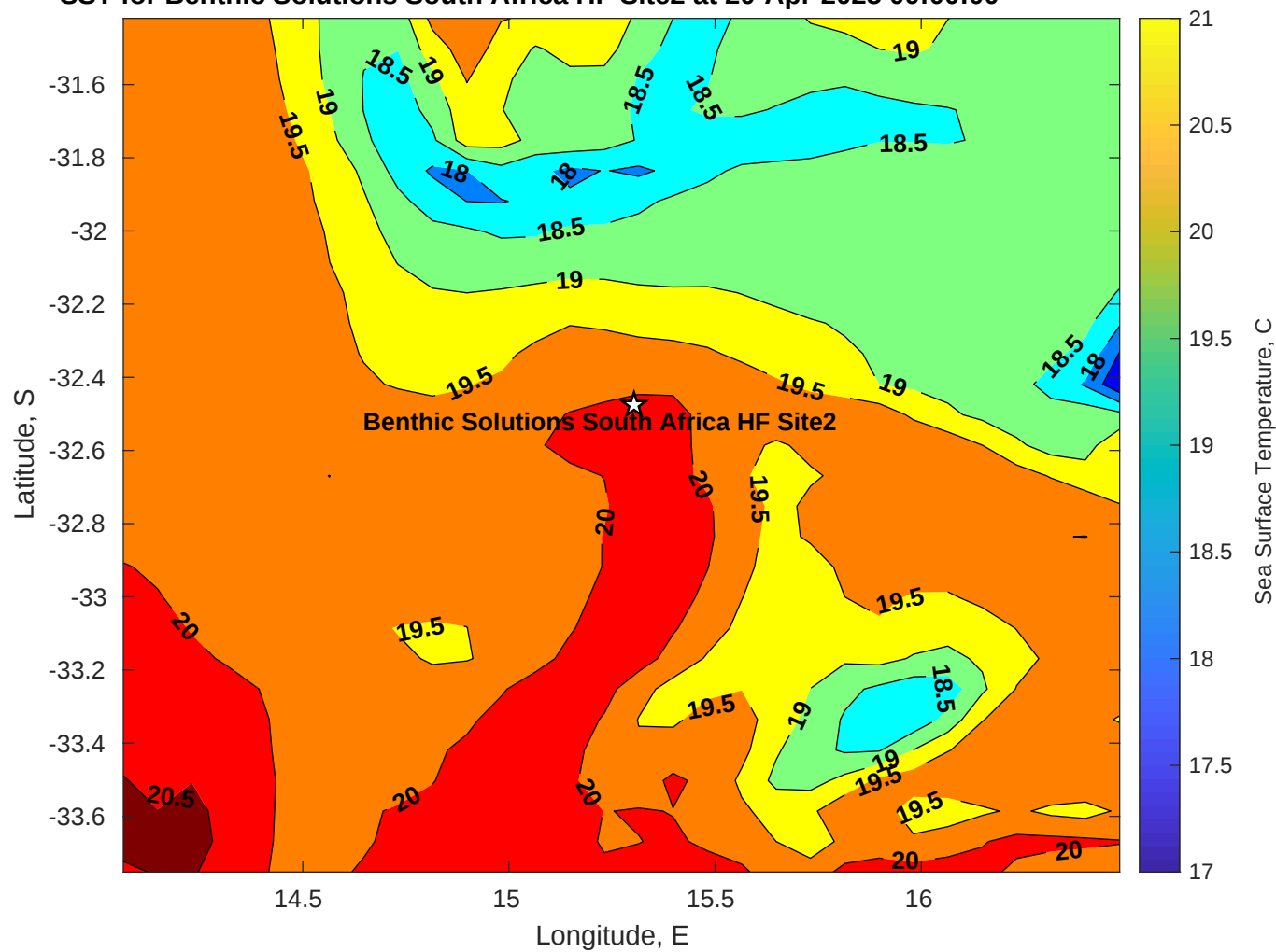
SST for Benthic Solutions South Africa HF Site2 at 20-Apr-2025 00:00:00
