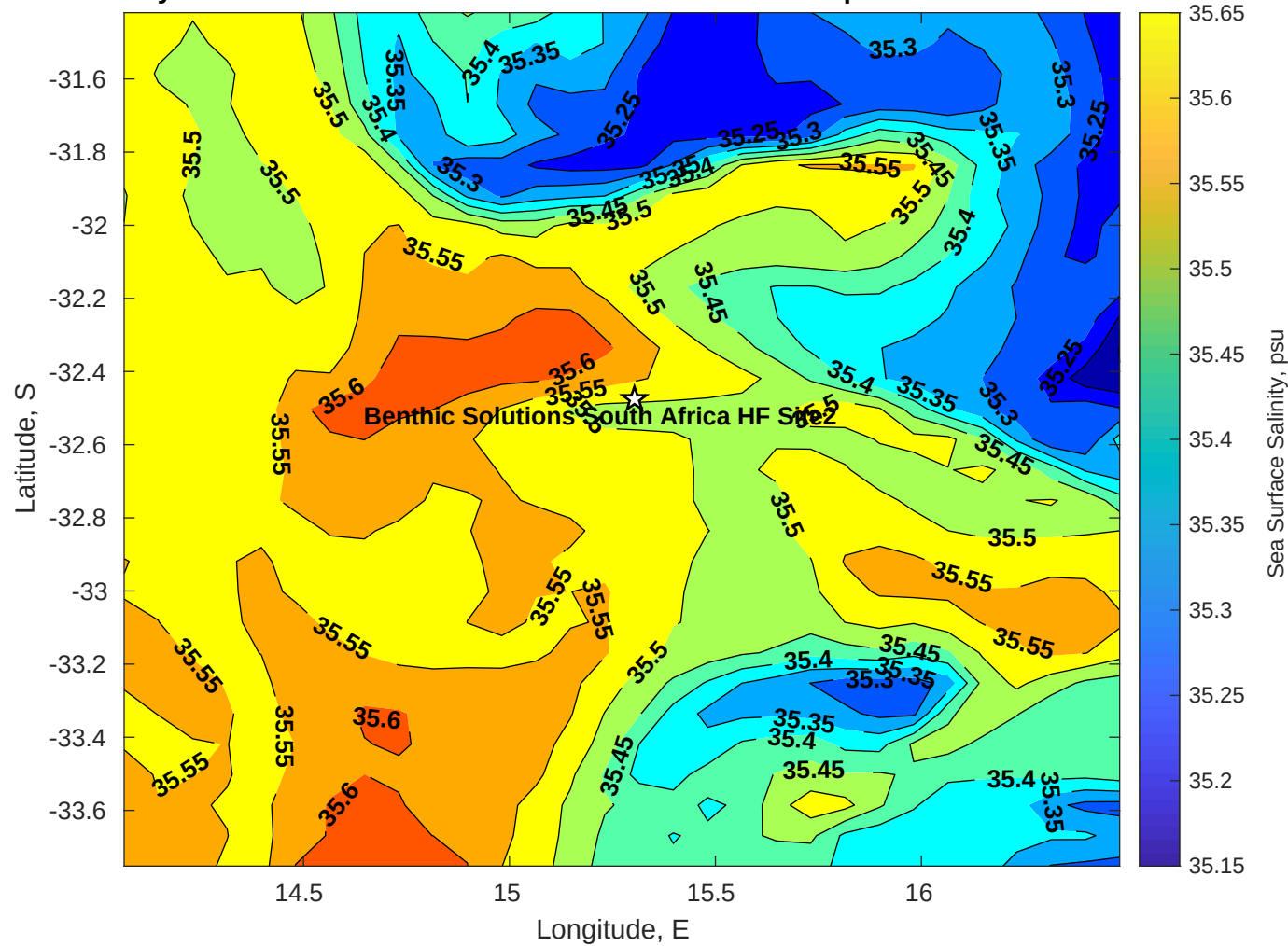
Surface Salinity for Benthic Solutions South Africa HF Site2 at 20-Apr-2025 00:00:00
