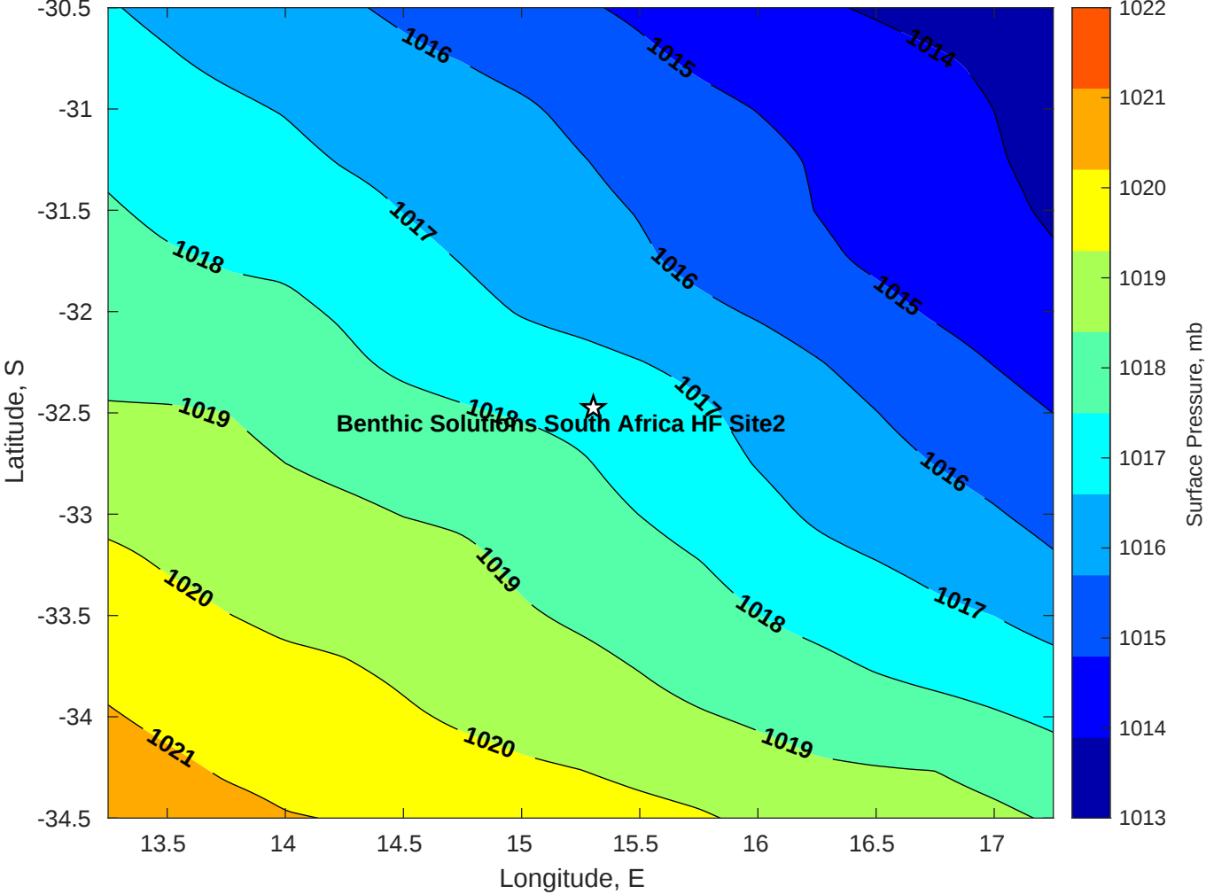
Surface Pressure (mb) for Benthic Solutions South Africa HF Site2 at 21-Apr-2025 00:00:00
