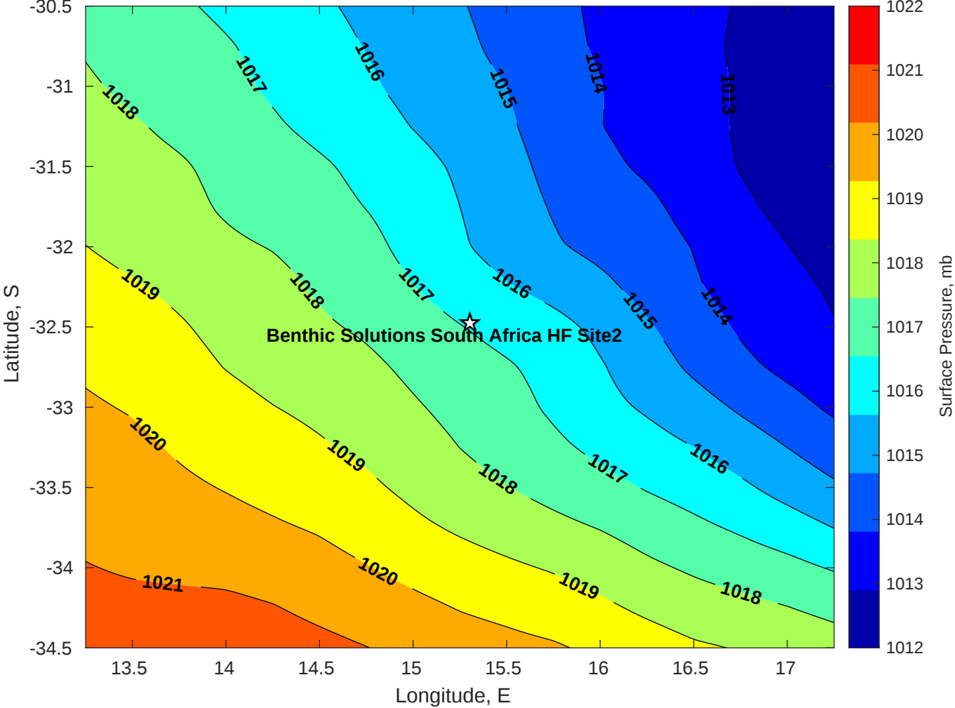
Surface Pressure (mb) for Benthic Solutions South Africa HF Site2 at 22-Apr-2025 00:00:00
