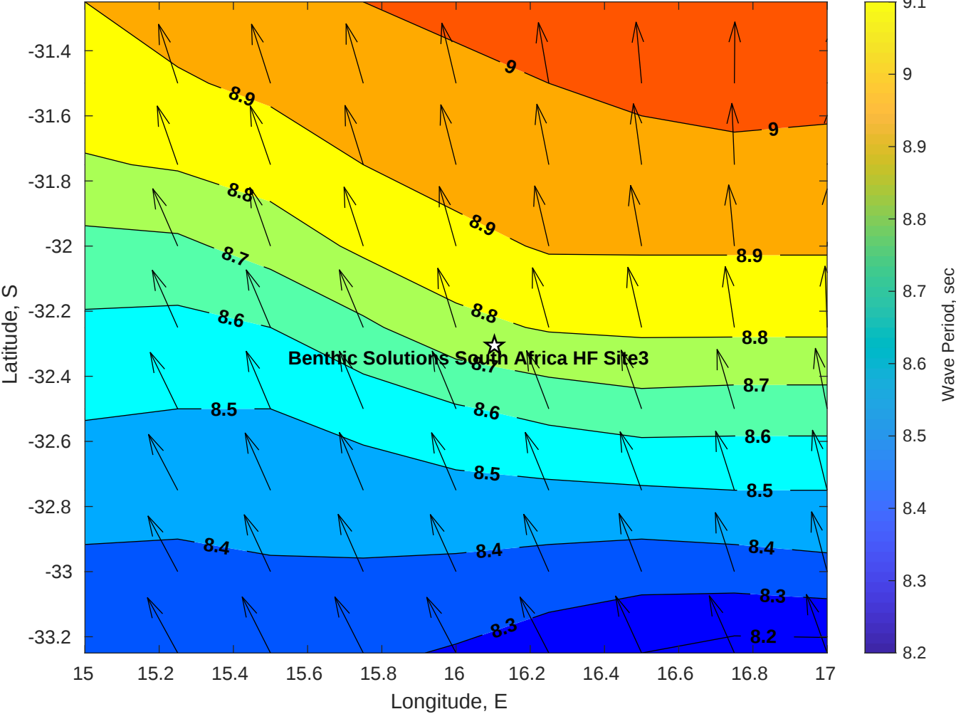
Wave Period (sec) for Benthic Solutions South Africa HF Site3 at 21-Apr-2025 09:00:00
