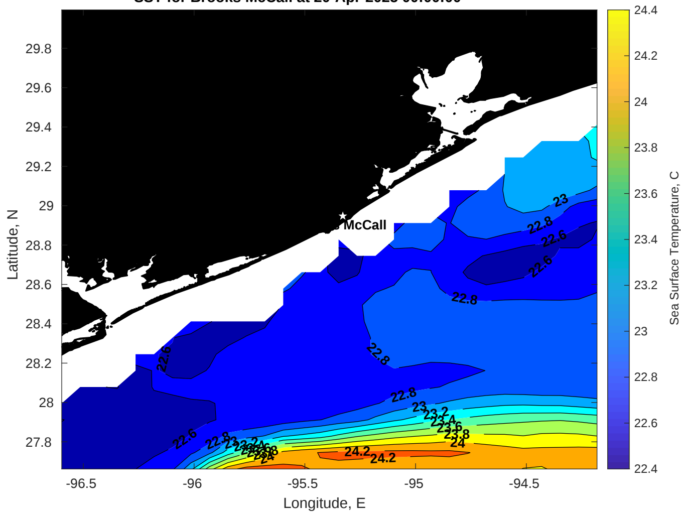
SST for Brooks McCall at 20-Apr-2025 00:00:00
