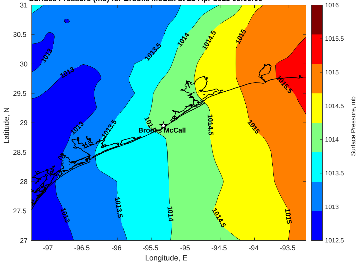
Surface Pressure (mb) for Brooks McCall at 21-Apr-2025 00:00:00
